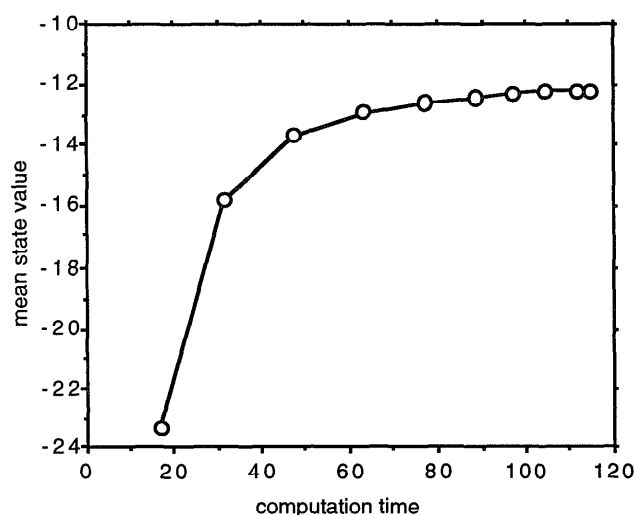
Figure 2: Anytime improvement in plan quality with multi-step policy iteration for the grid world example of figure 1. The single-step algorithm is started at time zero and the first circle marks the point at which it converges and the multi-step algorithm begins. Each circle after that represents a new iteration of the multi-step algorithm. The iterations are closer together near convergence because of previous caching of multi-step transition probabilities and payoffs. Computation time is in cpu seconds.
