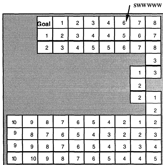
Figure 3: Multi-step policy at convergence. Each cell (or state) contains the length of the action sequence to take from that state before sensing again. One of the action sequences is shown as an example.
