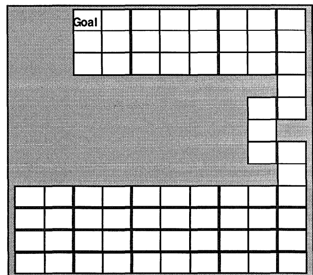
Figure 1: In this simple grid world, the robot tries to minimize the combined cost of sensing and hitting walls on its way to the goal.
