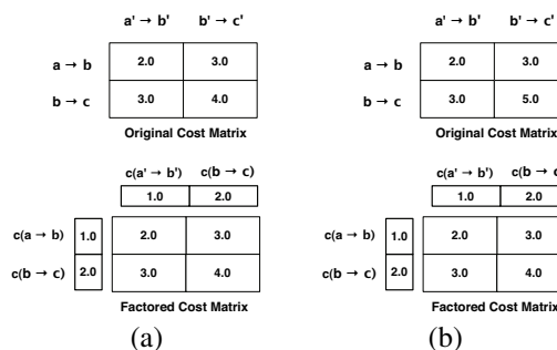
Figure 1: Example cost factoring: Each cell of the matrix is a local configuration composed of two projections (the row and column of the cell). In (a), the top matrix is an example cost matrix, which specifies the cost of each local configuration. The bottom matrix represents our factored estimates, where each entry is the sum of the configuration projections. For this example, the actual cost matrix can be decomposed exactly into two projections. In (b), the top cost matrix cannot be exactly decomposed along two dimensions. Our factored cost matrix has the property that each factored cost estimate is below the actual configuration cost. Although our factorization is no longer tight, it still can be used to produce an admissible heuristic.
