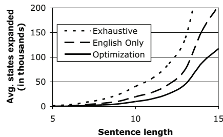
Figure 3: Parsing efficiency results show that the use of a suitable heuristic improves performance substantially, and both projections are required to maximize performance.
