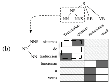
Figure 2: (a) A tree-to-tree transducer rule. (b) An example training sentence pair that yields rule (a).
