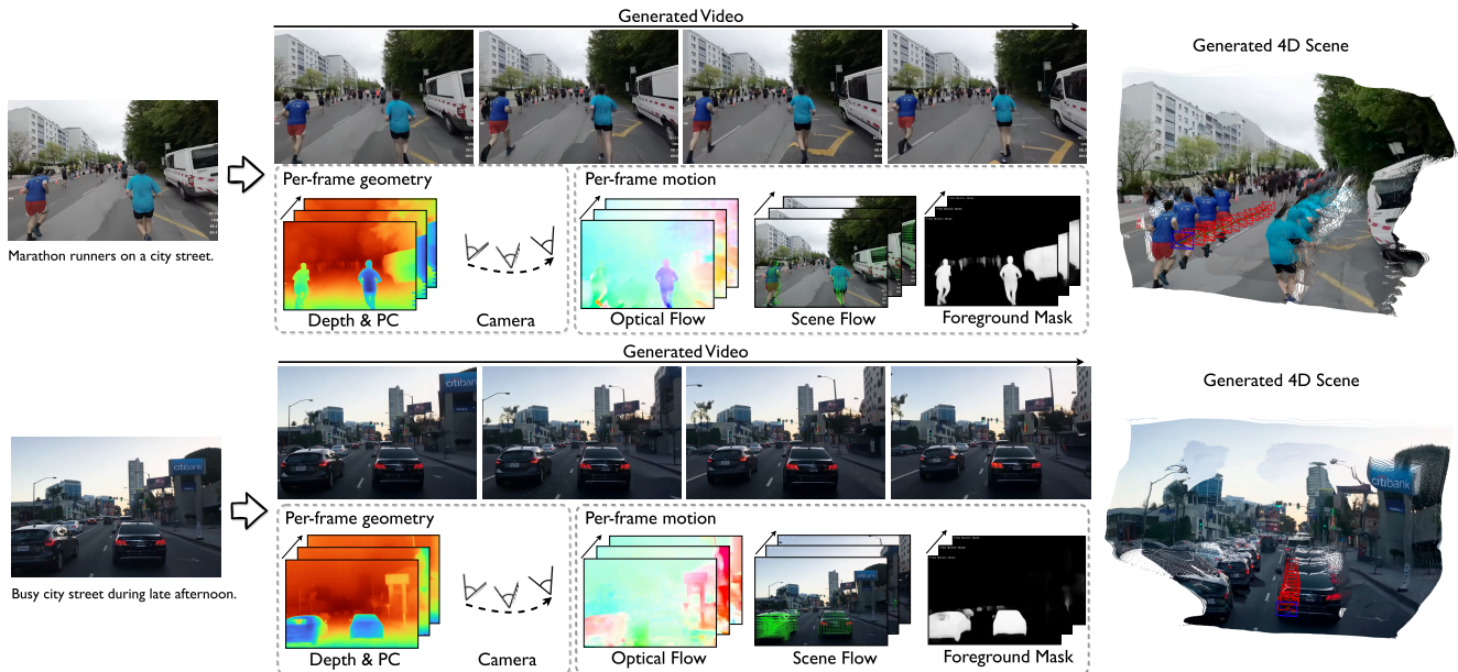
Figure 1. End-to-end 4D generation. Given a text prompt and a single input image (left), WorldReel generates a video (center) together with explicit 4D scene representations: per-frame geometry (depth + point cloud) with calibrated camera poses, and per-frame motion (optical flow, scene flow) with object masks (bottom panels). The rendered 4D scenes (right) exhibit consistent structure over time, even under non-rigid dynamics, illustrating spatiotemporal consistency and tight coupling of appearance, geometry, and motion.
