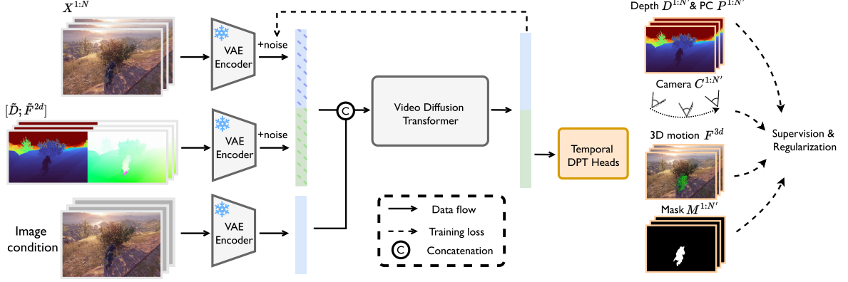
Figure 2. Overview of WorldReel. We augment a video diffusion transformer with a geo-motion latent (from RGB and 2.5D cues such as depth/optical flow) to inject a 4D inductive bias for spatio-temporal consistency. A temporal DPT decoder is trained with direct supervision and regularization to predict unified 4D outputs (depth/point cloud, calibrated camera, 3D scene flow, and masks).
