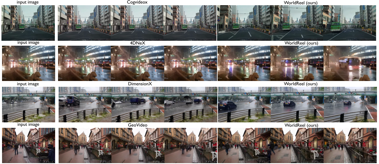
Figure 3. Qualitative image-to-video comparison on in-the-wild scenes. Given a single input image (left), we show sampled frames from videos generated by 4DNeX [10], DimensionX [52], GeoVideo [3], and WorldReel (ours). Prior methods often exhibit geometry drift and motion inconsistencies (e.g., warped facades, misaligned vehicles), while our results better preserve scene layout and maintain coherent camera and non-rigid dynamics. See the supplementary for prompts, full videos for all methods, and additional comparisons.
