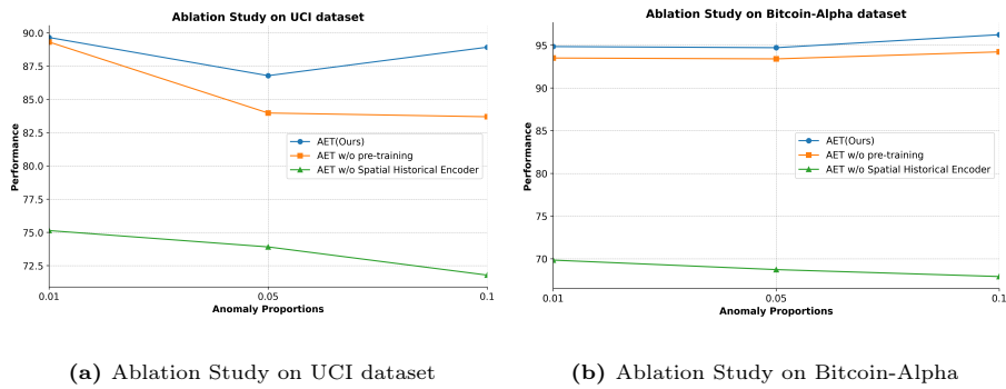
Fig. 4. Ablation Study
