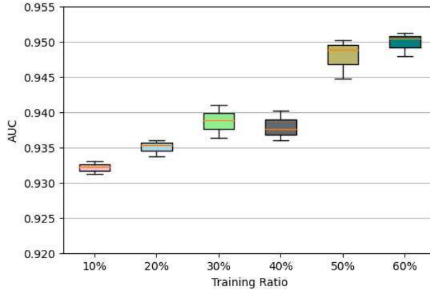
Fig. 3. AUC results on Bitcoin-Alpha with different training ratios
