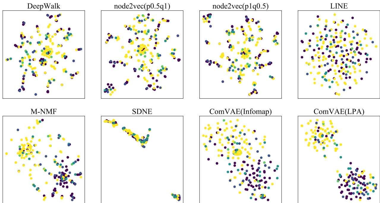
FIGURE 4. Visualization results on the Washington dataset.
