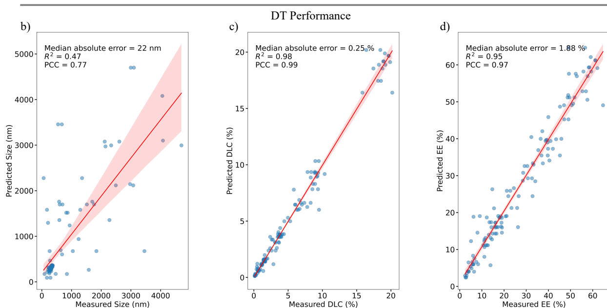
Figure 3. a) summarizes the accuracy (median absolute error, R^2 , and Pearson's correlation coefficient) of the eight, three-output machine learning regressors for predicting particle size, drug loading capacity (DLC), and encapsulation efficiency (EE). Three models, including decision tree (DT), random forest (RF), and extreme gradient boosting (XGB), exhibit high and comparable predictive accuracy. For simplicity and efficiency, the decision tree model was selected due to its straightforward structure and high training speed. The accuracy of the decision tree model is visualized in the scatter plots for b) Size, c) DLC, and d) EE predictions.
