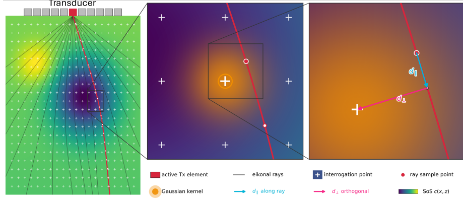
Fig. 1. For each active array element, rays are traced through the current SoS field c(x, z) . Nearby autofocus targets accumulate arrival-time estimates via a Gaussian kernel, with along-ray and orthogonal offsets d_{\parallel} and d_{\perp} defining the time correction and deposition weight.
