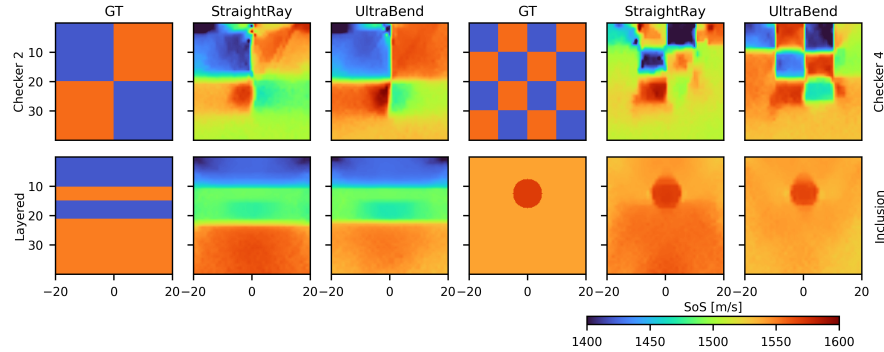
Fig. 3. Speed-of-sound reconstructions from k-Wave simulations with known numerical phantoms. Each triplet shows ground truth (GT), StraightRay, and UltraBend. Spatial dimensions are in mm.
