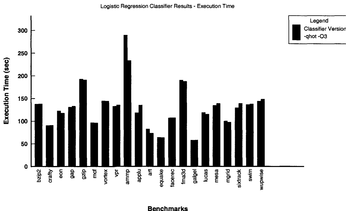
Figure 5.4: Comparison of the execution time using the classifier and the baseline.
