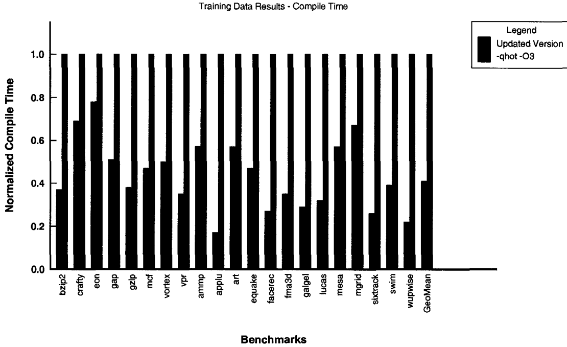
Figure 5.1: Comparison of the compile time for the new version with the set of heuristics after training vs the original version at -qhot -O3 optimization level
