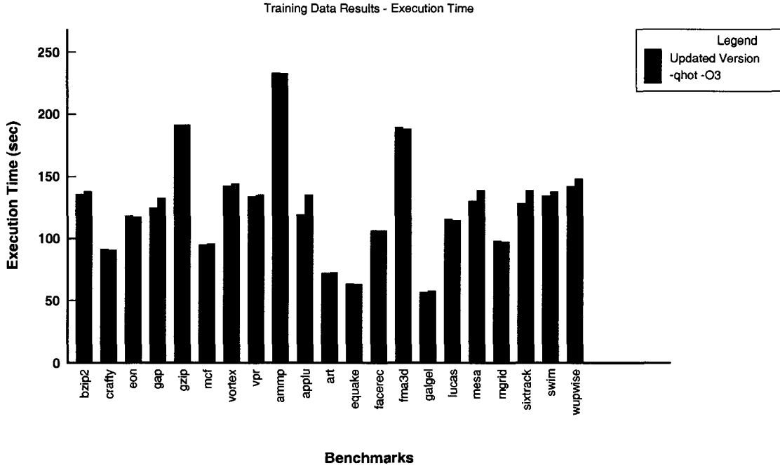
Figure 5.2: Comparison of the execution time for the new version with the set of heuristics after training vs the original version at -qhot -O3 optimization level
