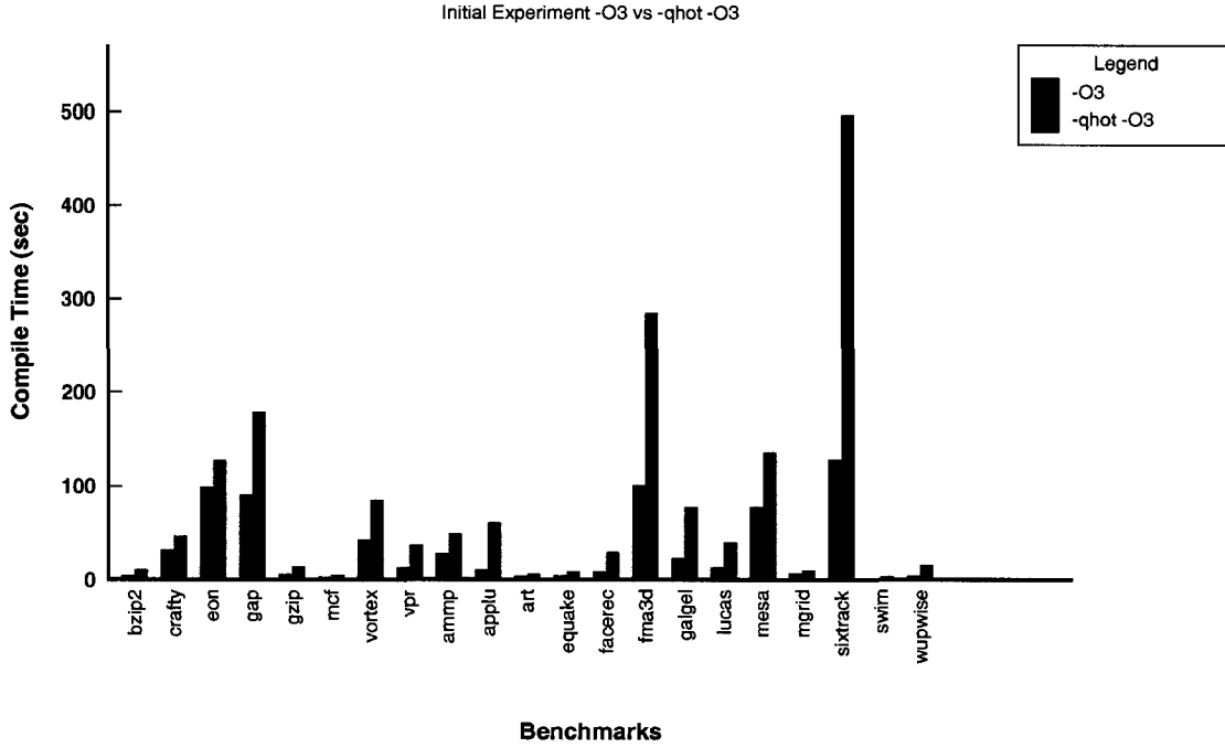
Figure 2.1: Comparison of the compile time for two optimization levels (-O3 and -qhot -O3) on SPEC2000 benchmarks.
