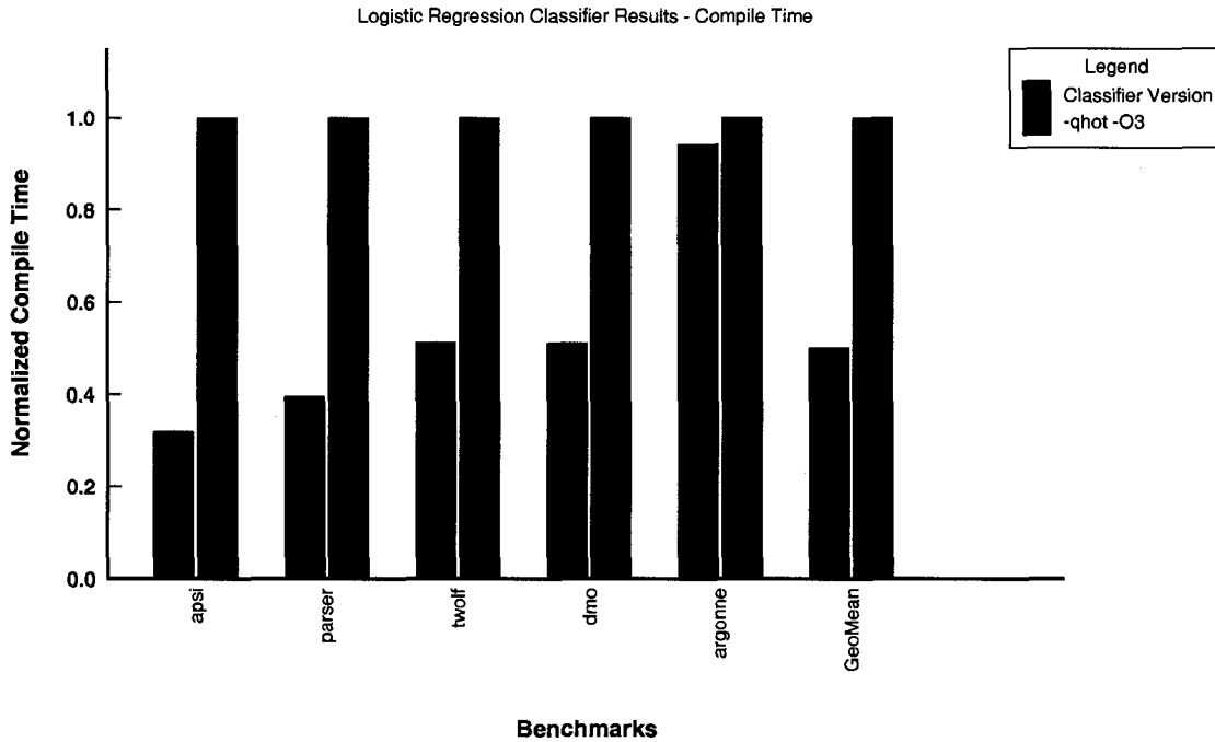
Figure 5.5: Comparison of the compile time using the classifier and the baseline.
