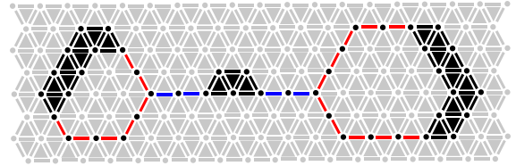
Fig. 4 A simplicial stack F with two values (0 in gray and 1 in black, red, and blue) on a subset of a normal 2-pseudomanifold. In blue and red, the separating faces. In red, the biconnected faces.
