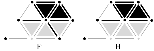
Fig. 3 Two stacks F and H with two levels: altitude 0 (faces in light gray) and altitude 1 (faces in black). The stack H is an elementary collapse of F (at altitude 1). But F has three minima whereas H has only two. Thus, \min(H) is not an extension of \min(F) .
