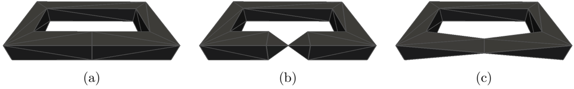
Fig. 2 (a): A normal pseudomanifold, which is a torus, (b): A pseudomanifold, which is a pinched torus, and where the pinch face is a vertex, (c): A pinched torus where the pinch face is a segment. This is not a pseudomanifold.
