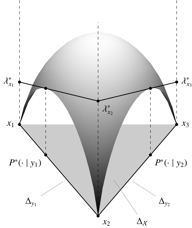
Figure 3: The worst-case optimal strategy for the quizmaster in the Monty Hall game with logarithmic loss, as characterized by Theorem 3. The triangular base is the full simplex \Delta_X , on which the entropy function H_L is defined (this is the grey dome); the points labelled x_1 , x_2 and x_3 are the elements of this simplex putting all mass on that single outcome; and the line segments \Delta_{y_1} and \Delta_{y_2} are the subsets of \Delta_X consisting of all distributions on y_1 and y_2 respectively. Restricted to the domain \Delta_{y_1} , the vector \lambda^* defines a linear function (having height \lambda_x^* at each x \in X ) that is a supporting hyperplane to H_L at P^*(\cdot | y_1) (and similar for y_2 ). Note that when the linear function defined by \lambda^* is extended to all of \Delta_X , it may go below H_L there, but not in \Delta_{y_1} or \Delta_{y_2} .
