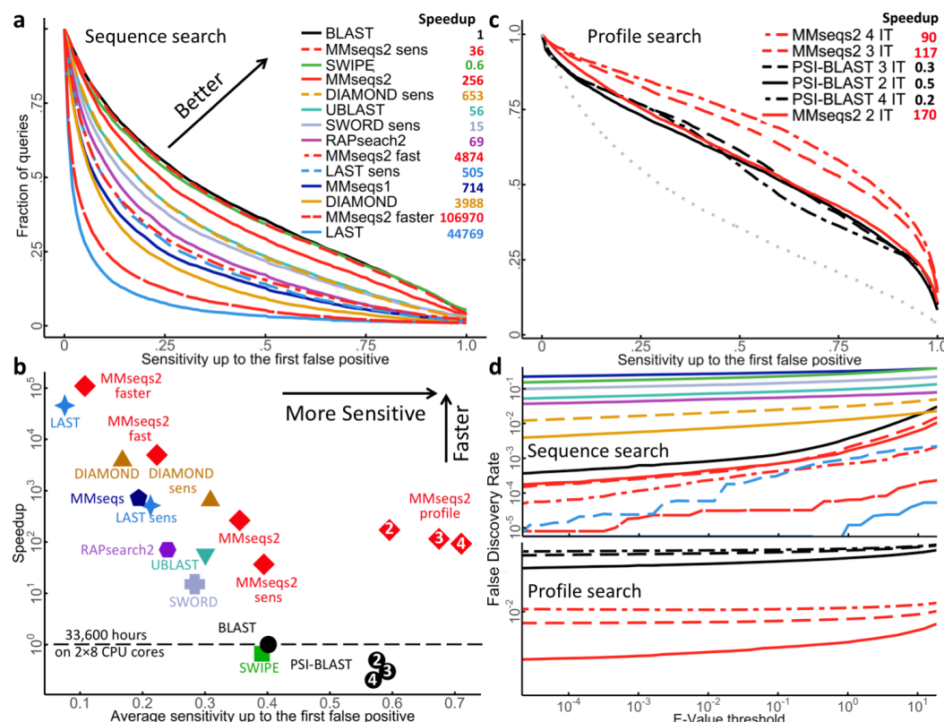
Figure 2: MMseqs2 pushes the boundaries of sensitivity-speed trade-off. a Cumulative distribution of Area under the curve (AUC) sensitivity for all 6370 searches with UniProt sequences through the database of 30.4 M full-length sequences. Higher curves signify higher sensitivity. Legend: speed-up factors relative to BLAST, measured on a 2×8 core 128 GB RAM server using a 100 times duplicated query set (637 000 sequences). Times to index the database have not been included. MMseqs2 indexing takes 11 minutes for 30.3M sequences of avg. length 342. b Average AUC sensitivity versus speed-up factor relative to BLAST. White numbers in plot symbols: number of search iterations. c Same analysis as in a , for iterative profile searches. d False discovery rates for sequence and profile searches. Colors: as in a (top) and c (bottom).
