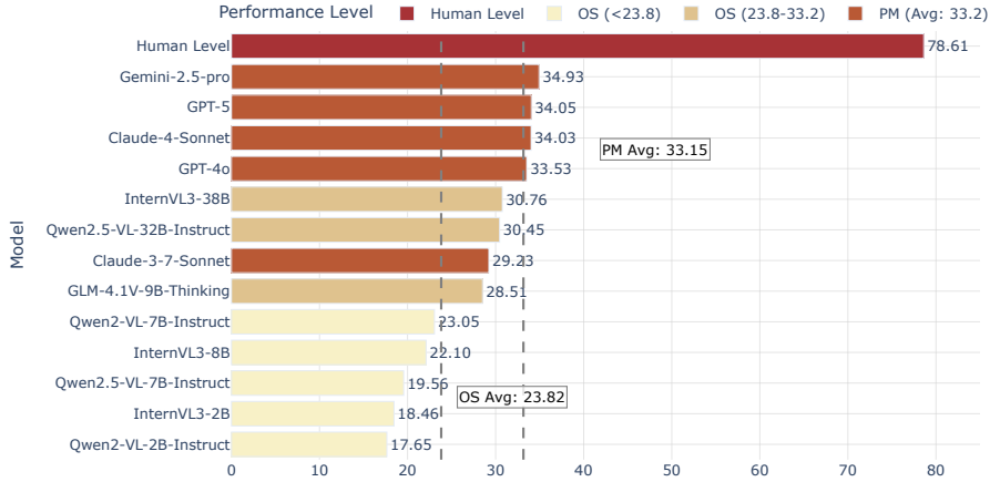
Figure 5: Overview Comparison of human performance and 13 VLMs on GTR-Bench. The best model (Gemini-2.5-Pro, 34.93%) remains far below human performance (78.61%). Dashed lines indicate average performance: OS Avg (23.82) < PM Avg (33.15) \ll Human (78.61%).
