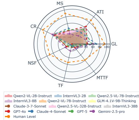
Figure 6: Task performance of GTR-Bench
