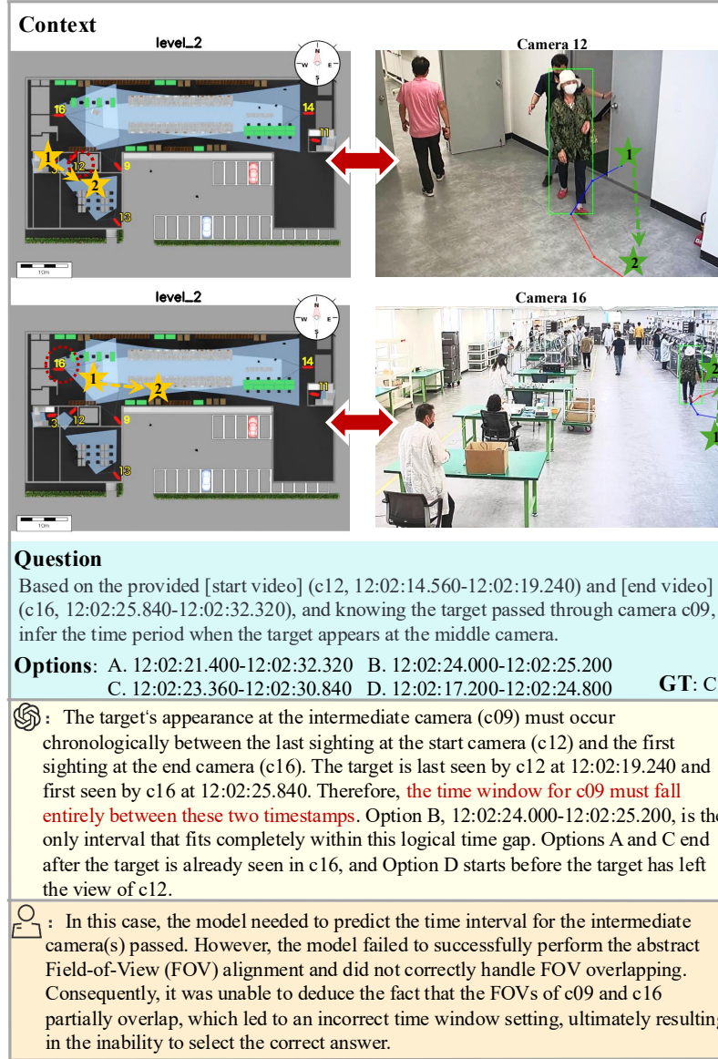
Figure 15: FoV Misinterpretation. The model fails to perceive the overlap between the Abstract FoVs of adjacent cameras on the map, leading to incorrect temporal or spatial reasoning.
