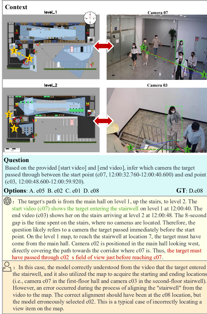
Figure 14: FoV to Map Misalignment. The model correctly identifies the semantic location ("stairwell") from the concrete video view but fails to map it to the geometric location on the map.
