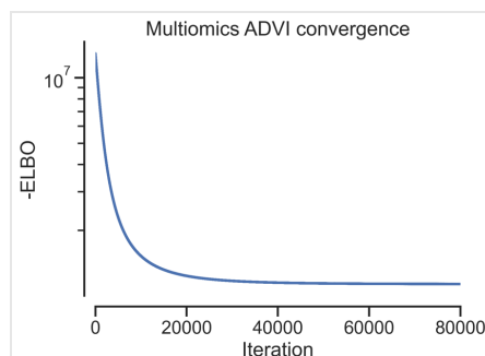
Figure 2: Optimization of the ELBO score.
