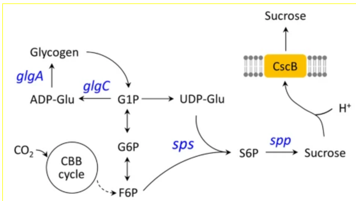
Figure 5: Engineered pathways for sucrose production. This diagram highlights the sucrose production pathway engineered into S. elongatus . Particularly the CscB gene which allows for sucrose to be exported from the cell. We can visualize how some suggested modifications from the FCC plot may affect this pathway, such as the under expression of GLCS3 reaction representing the glgA gene.
