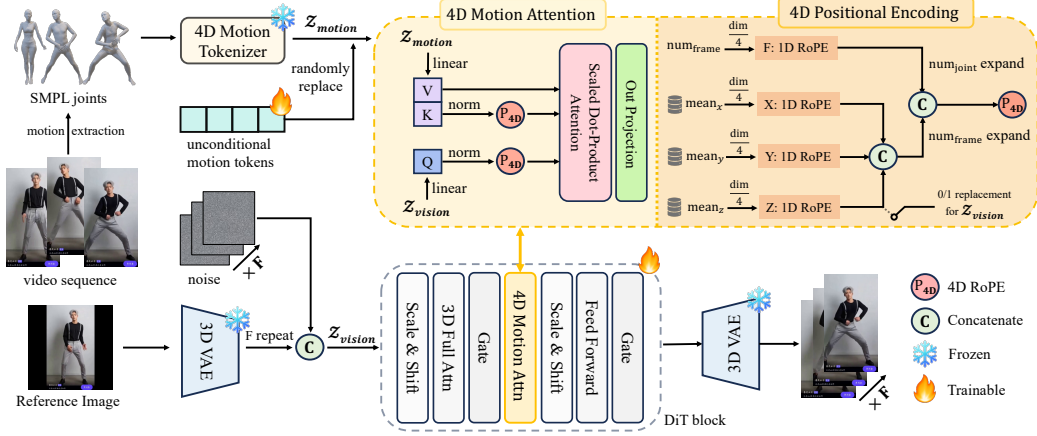
Figure 4: Architecture of MTVCraft-6B. Based on the video DiT model, we design unique 4D motion attention to leverage 4D motion tokens as context for vision generation. To enhance spatial-temporal relationships, we apply 4D RoPE over (t, x, y, z) coordinates to attention keys and queries.
