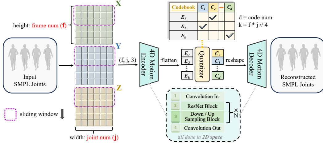
Figure 3: Architecture of 4DMoT. An encoder-decoder framework learns spatial-temporal latent representations of SMPL joint coordinates, and a vector quantizer learns 4D compact yet expressive tokens in a unified space. All operations are in 2D space along the frame and joint axes.
