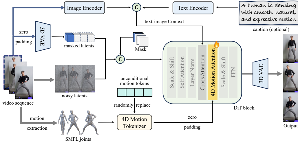
Figure 6: Architecture of MTVCraft-18B. To demonstrate the versatility of our approach and further improve performance, we scale the model to a larger DiT and enable joint text-motion control. Here, zero-padding aligns the motion token dimension with the DiT hidden dimension.
