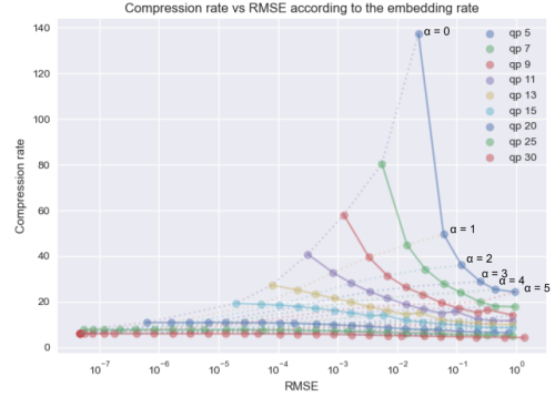
Fig. 7: Mean compression rate as a function of the RMSE for various qp and \alpha , for the entire Stanford database [12].
