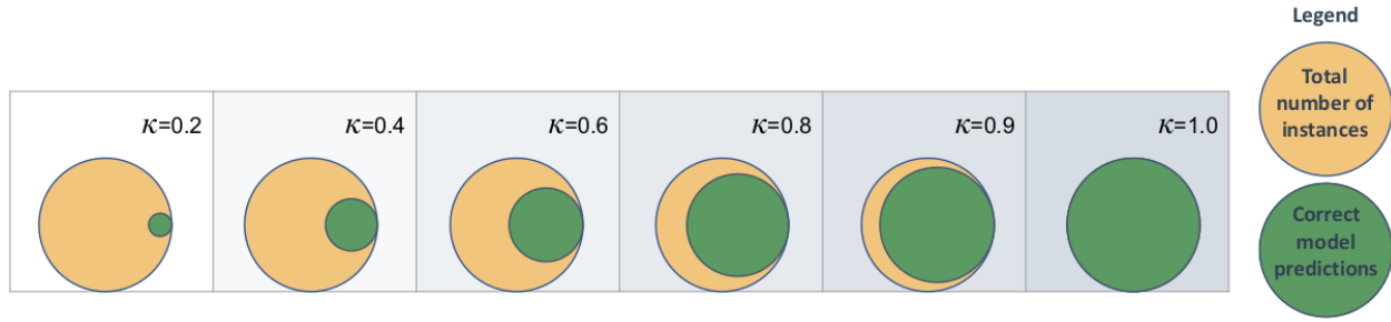
Figure A.5: Kappa values for different degrees of agreement. The illustration is based on [86, Figure 2].
