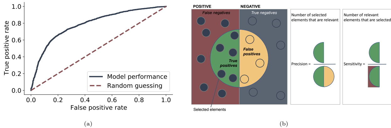
Figure A.4: (a) A receiver operating characteristic curve, and (b) A visual representation of the sensitivity, eq. (A.4), and the precision, eq. (A.5), highlighting the trade-off between the two.
