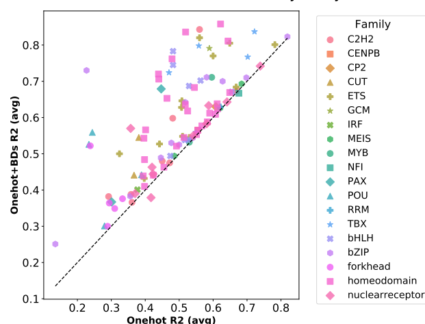
Scatter Plot of Onehot+BDs R^2 vs Onehot R^2 by Family
