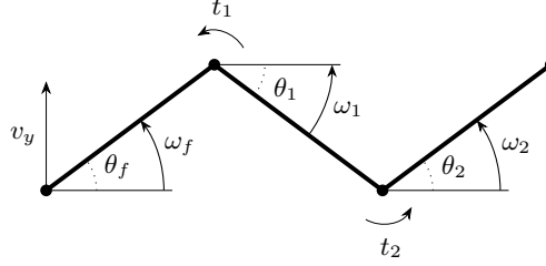
(a) Swimmer schematic.
