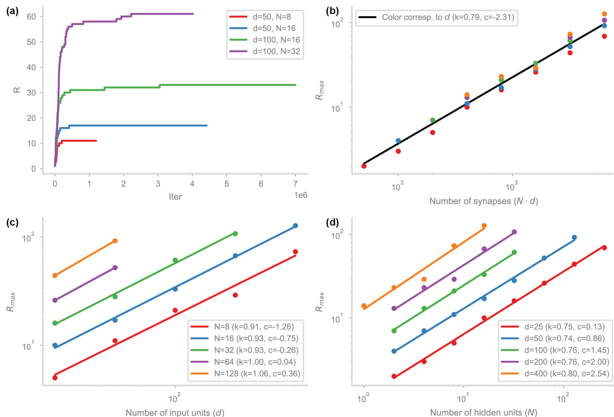
Figure 5. Curriculum training and empirical capacity. (a) The value of R used over the course of curriculum training for four different network sizes. R is incremented once the network achieves an accuracy > 0.99 . Training is considered converged when the value of R is not incremented for at least 1 million iterations. (b) The final value of R after curriculum training (i.e. network capacity) as a function of the number of plastic synapses in the network, plotted on a log-log scale. The color of the points corresponds to the number of input
