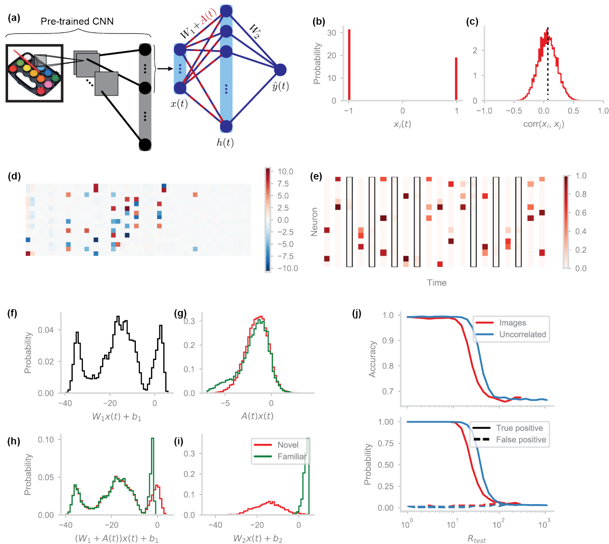
Figure 8. HebbFF performance on real-world images. (a) Network architecture for familiarity detection of real-world images. The activity of the penultimate layer of a convolutional neural network (ResNet18, pre-trained on ImageNet) is downsampled and passed to the HebbFF network ( d = 50, N = 16 ) for familiarity detection. Only the HebbFF portion of this network is trained, via curriculum training. (b) Distribution of inputs x(t) to HebbFF. After down-sampling by extracting the first 50 units of the CNN, the activity is centered at zero and binarized. (c) Histogram of the correlations between all pairs of input stimuli x(t) . On average (vertical dashed line) the correlation is slightly positive. (d-h) Same plots as Fig 4(f,c,i,j,m), respectively ( R_{\text{train}} = R_{\text{test}} = 12 ). (j) Generalization performance, compared to a network of the same size trained on uncorrelated binary random vectors, is lower due to correlations in the input images.
