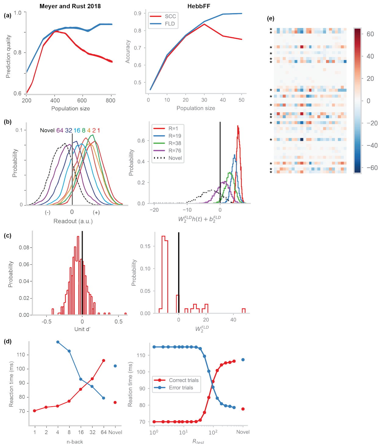
Figure 7. Comparison to IT cortex data. (a) Left: neurons from the IT cortex used to predict the behavioral outputs of a monkey performing continual familiarity detection, decoded using the Fisher linear discriminant (FLD, blue) or spike count classifier (SCC, red). Right: units from the hidden layer of a trained HebbFF network (trained with an unconstrained readout W_2 rather than uniform) used to detect familiarity obtained from SCC and FLD decoders. In both cases, the number of neurons/units available to the decoder was varied, added in order of increasing weight according to the FLD decoder. While the FLD decoder accuracy saturates, the SCC decoder accuracy peaks and begins to decline as more neurons/units are included in the decoder. (b) Distribution the FLD decoder output for IT cortex neurons (left) and HebbFF hidden units (right) for novel stimuli, and familiar stimuli at varying delay intervals. In both cases, the distribution shifts towards lower values as delay interval increases. For HebbFF, the distribution gets narrower for shorter delay intervals due to saturation in the hidden layer units. (c) Distribution of the FLD decoder weights for decoding IT cortex data (left) or HebbFF hidden unit activity (right). In both cases, the majority of output weights are negative, with some positive values.
