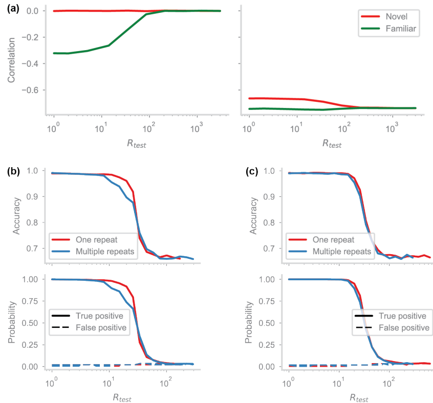
Figure S4. Idealized and HebbFF model differences. (a) Correlation between the hidden layer input currents due to static and plastic synapses for the idealized model (left) and HebbFF (right) for novel (red) and familiar (green) stimuli as a function of delay interval ( d = 25, N = 32 ). In the idealized model, due to the split static and plastic synapses, the currents are uncorrelated for novel stimuli and familiar stimuli at long delay intervals. At short intervals, the two input currents are anti-correlated, which enables repetition suppression. In the HebbFF model, there is anti-correlation in both cases, although there is still less anti-correlation for novel stimuli. (b) Performance of the idealized network on the continual familiarity detection task with familiar stimuli repeated either exactly once, as used throughout this work (red), or multiple times (blue). Since there is exactly zero hidden unit activity for a familiar stimulus it does not get reinforced in memory, and less likely to be recognized on its second and subsequent repetitions. (c) The HebbFF network, trained to maximum capacity on the single-repeat task does not suffer any loss in performance due to multiple repeats.
