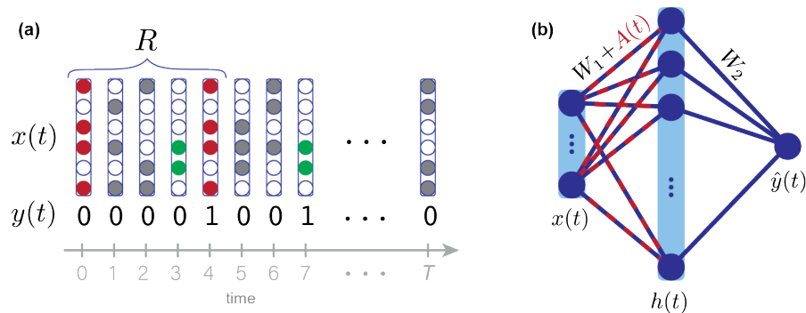
Figure 1. Continual familiarity detection task and HebbFF model. (a) The continual familiarity detection task. Given a continual stream of stimuli x(t) , the desired output is y(t) = 1 if the stimulus has appeared previously and y(t) = 0 otherwise. For a given dataset, repeat stimuli always appear at an interval R after their first presentation. Although the task is continual, for the purposes of network training we use a finite-duration trial of length T \gg R . (b) The HebbFF network architecture. A feedforward layer is endowed with ongoing Hebbian plasticity, the parameters of which are optimized using stochastic gradient descent. The hidden units are linearly read out to produce the network's estimate of familiarity \hat{y}(t) .
