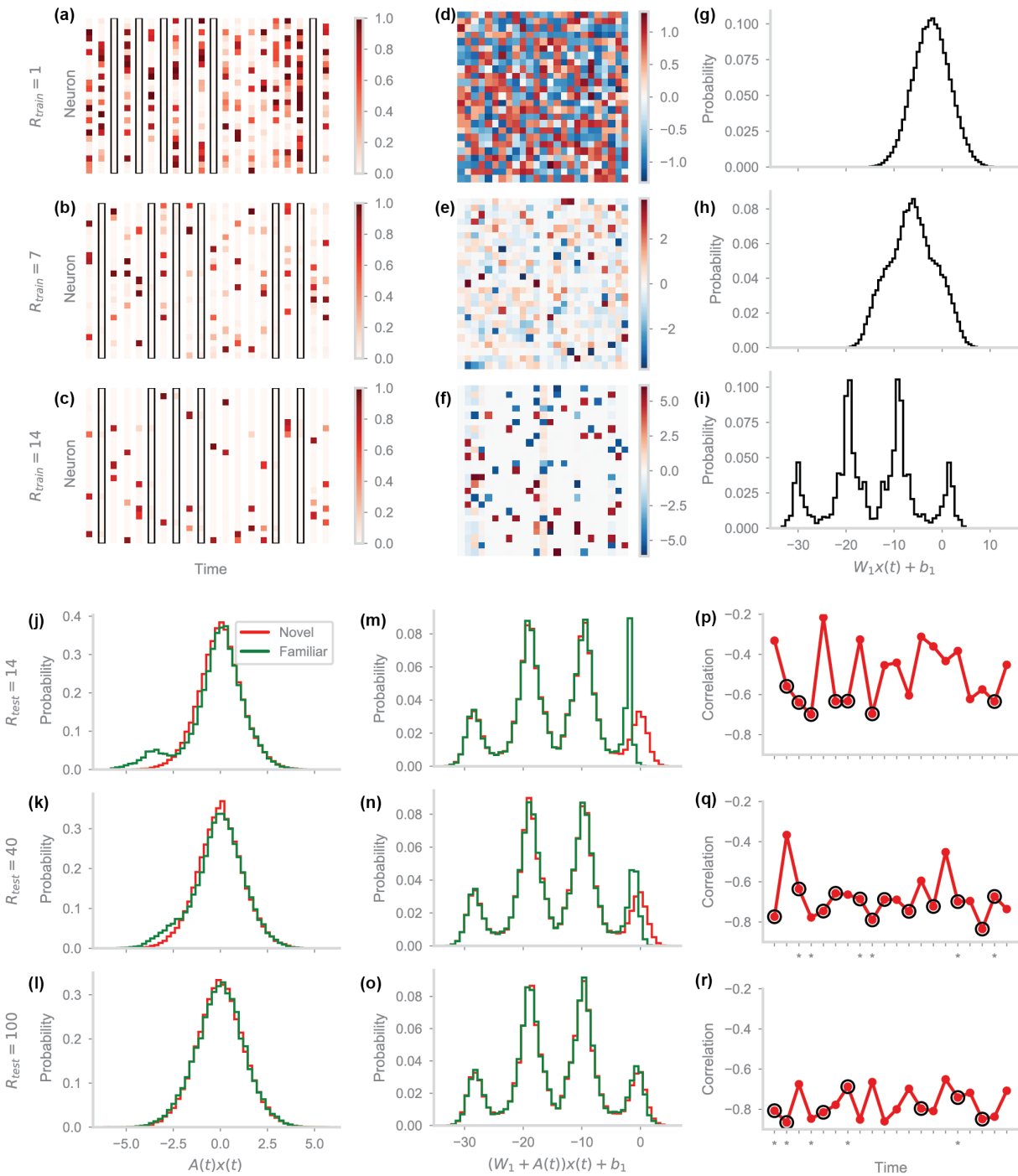
Figure 4. Storage and readout mechanism. (a-c) Hidden layer activity h(t) over 20 consecutive timesteps for networks with input dimension d = 25 and N = 25 hidden units, trained on datasets with R = 1, 7 , or 14 , respectively. Familiar stimuli (black rectangles) cause silencing i.e. repetition suppression of hidden layer activity. Activity for novel stimuli becomes sparser for networks trained with larger R . (d-f) Static weight matrix W_1 of the networks from (a-c). The weight matrix becomes sparser, and individual weight magnitudes increase for networks trained with larger R , enabling more sparse activity in the hidden layer for novel stimuli. (g-i) Distributions of input current into the hidden layer due to the static component of the synapses, i.e. the matrix W_1 and bias b_1 , for the networks from (a-c). We do not distinguish familiar and novel stimuli since the current due to the static component is the same regardless of novelty. For networks trained with larger R , the distribution becomes multi-modal, with the number of modes equal (approximately) to the number of high-magnitude values per row of W_1 , plus one. Due to the bias, only the rightmost mode has the potential to produce firing rates that are significantly above zero. (j-l) Distributions of input current into the hidden layer due to the plastic component of the synapses, i.e. the matrix A(t) , for novel (red) and familiar (green) stimuli. We only consider the trained network from (c,f,i) and evaluate its behavior on test sets with R = 14, 40 , or 100 , corresponding to perfect, intermediate, and chance
