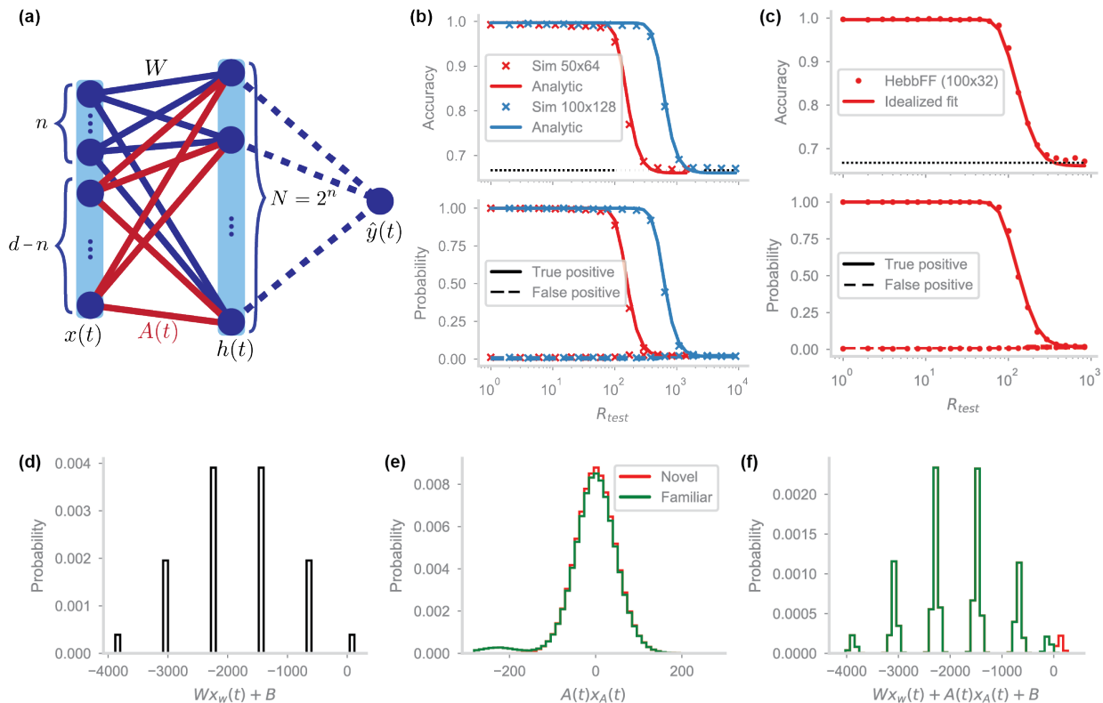
Figure 6. Idealized model. (a) The idealized HebbFF network architecture. In contrast to the original HebbFF network with a single effective matrix W_1 + A(t) , the input x(t) is effectively split into two sections of size n and D = d - n that serve as inputs into separate static and plastic synaptic matrices W_1 and A(t) , respectively ( Online methods ). The hidden layer size is N = 2^n . The readout unit outputs \hat{y}(t) = 1 whenever any of the hidden units is active. (b) The analytic calculation of network performance (solid line) matches simulation results for the idealized network (x's), shown for two different network sizes (red, blue). (c) A least-squares fit of the analytic performance curve of the idealized network to a trained HebbFF network of the same size for two network sizes. The idealized network has similar performance to the HebbFF model if its decay rate and bias are scaled appropriately: \lambda \approx 0.986 , b_1 \approx -4.771 (for all units) for d = 200 , N = 32 , and \lambda \approx 0.993 , b_1 \approx -4.771 for d = 200 , N = 32 . (d-f) Same as Fig 4(l,j,m), but for the idealized network ( D = 400 , N = 32 , R = 300 ).
