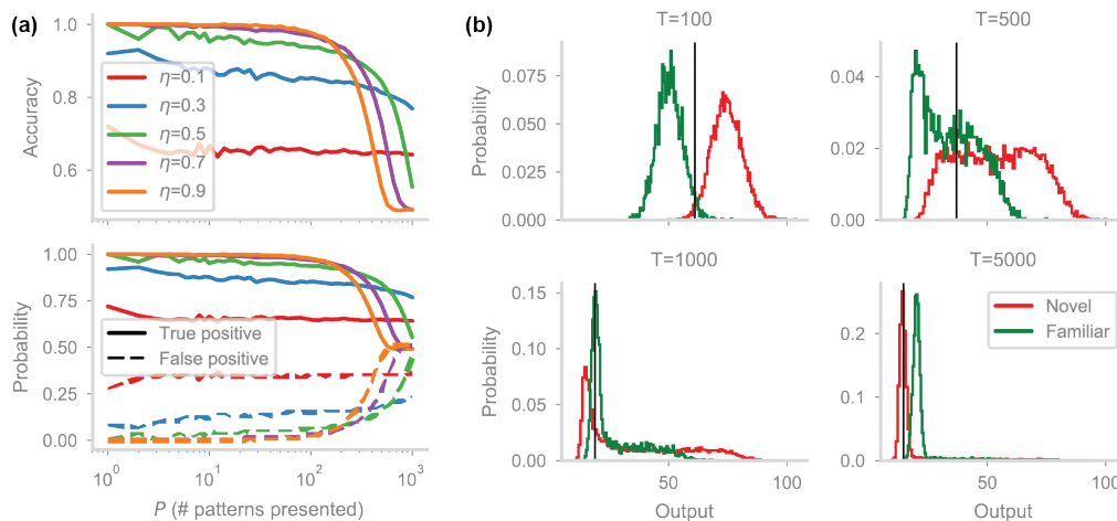
Figure S2. Validation of network from Bogacz and Brown (2003). (a) Performance of the anti-Hebbian network from (Bogacz and
