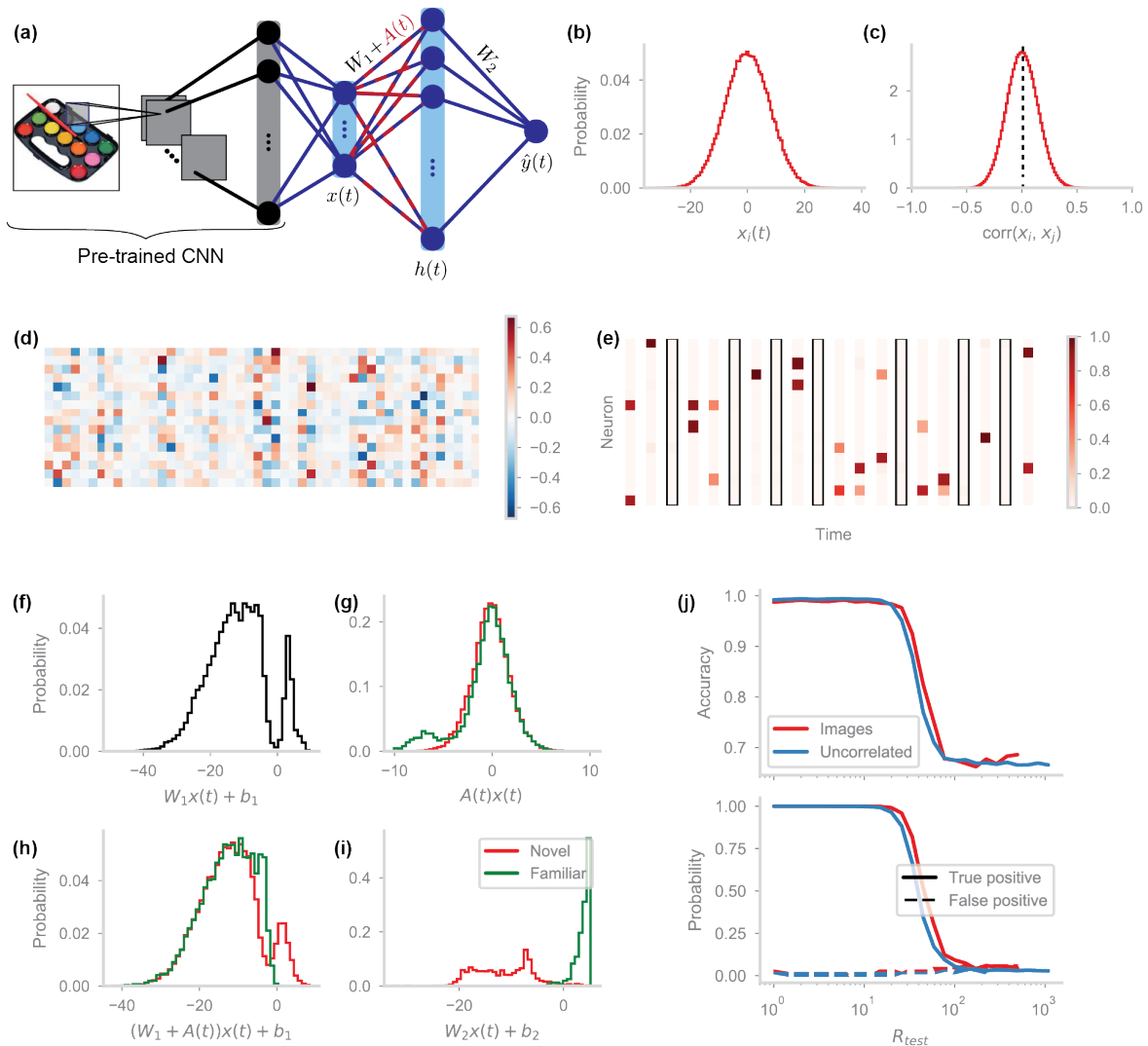
Figure S6. Performance on real-world images. Subplots as in Fig 8, but using a trained fully-connected linear layer to transform the activations of the CNN's penultimate layer into the inputs of HebbFF ( R_{\text{train}} = R_{\text{test}} = 19 ).
