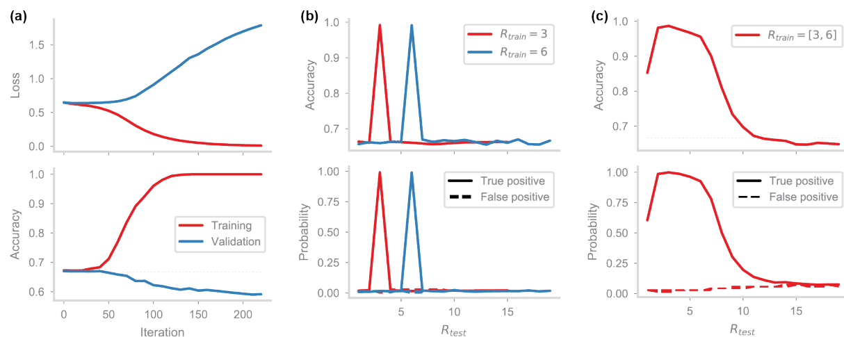
Figure 2. RNN performance on continual familiarity detection. (a) Training an LSTM ( d = 100 input dimension, N = 100 recurrent units) on a single dataset of a familiarity detection task ( T = 500 stimulus presentations, repeat interval R = 3 ). Although the loss (top) approaches zero and accuracy (bottom) approaches 1 on the training dataset (red curves), performance on a validation dataset (blue) with the same parameters fails to generalize even when tested in-distribution with the same R . (b) Training the RNN using "infinite data." New datasets, each with R = 3 , are generated at every epoch of training (red). Accuracy (top), as well as true positive and false positive probabilities (bottom) is shown as a function of the repeat interval on validation datasets. The same is repeated with another RNN using R = 6 (blue). The RNNs perform well in-distribution on datasets with the same repeat interval as used during training, but fail to generalize out-of-distribution to other repeat intervals. (c) Training the RNN with "infinite data," using datasets with both repeat intervals R = 3 and R = 6 . The RNN interpolates between the intervals – performance is high when tested on repeat intervals 3 \leq R \leq 6 – but fails to extrapolate. Performance quickly drops for longer repeat intervals, and even for shorter ones.
