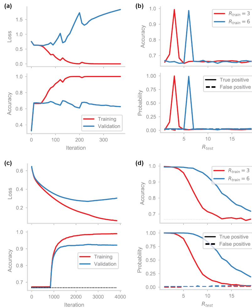
Figure S1. HebbFF and RNN comparison, matching total number of dynamic variables. (a,b) RNN performance as in Fig 2a-b, with d = 25 and N = 625 . (c,d) HebbFF performance as in Fig 3a-b, with d = 25 and N = 25 . The number of plastic synapses in the HebbFF network N * d = 625 is the same as the number of recurrent units in the RNN, matching the number of dynamic variables between the networks rather than the number of neurons. HebbFF still shows better generalization in both training scenarios.
