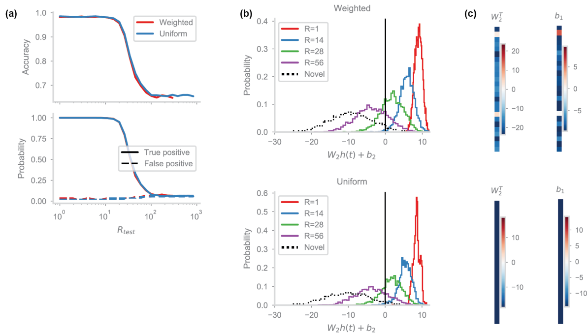
Figure S3. Comparison of uniform and trained readout. (a) Generalization performance of a trained HebbFF network ( d = N = 25 ) with a fully trainable readout matrix, i.e. a weighted average of the hidden layer activity (red) and a version where all the entries of the readout matrix are constrained to be equal, i.e. a scaled average of the hidden layer (blue). (b) Distributions of the output unit activity (prior to applying the nonlinearity) for a trained network, for several test values of R . The output distributions, as well as performance, are almost identical for both versions of the readout. (c) Examples of the W_2 readout matrix, as well as the bias b_1 for the weighted (top) and uniform (bottom) readouts. Values for both are negative, indicating a qualitatively similar readout mechanism. Note that the weight matrices are plotted transposed for visualization.
