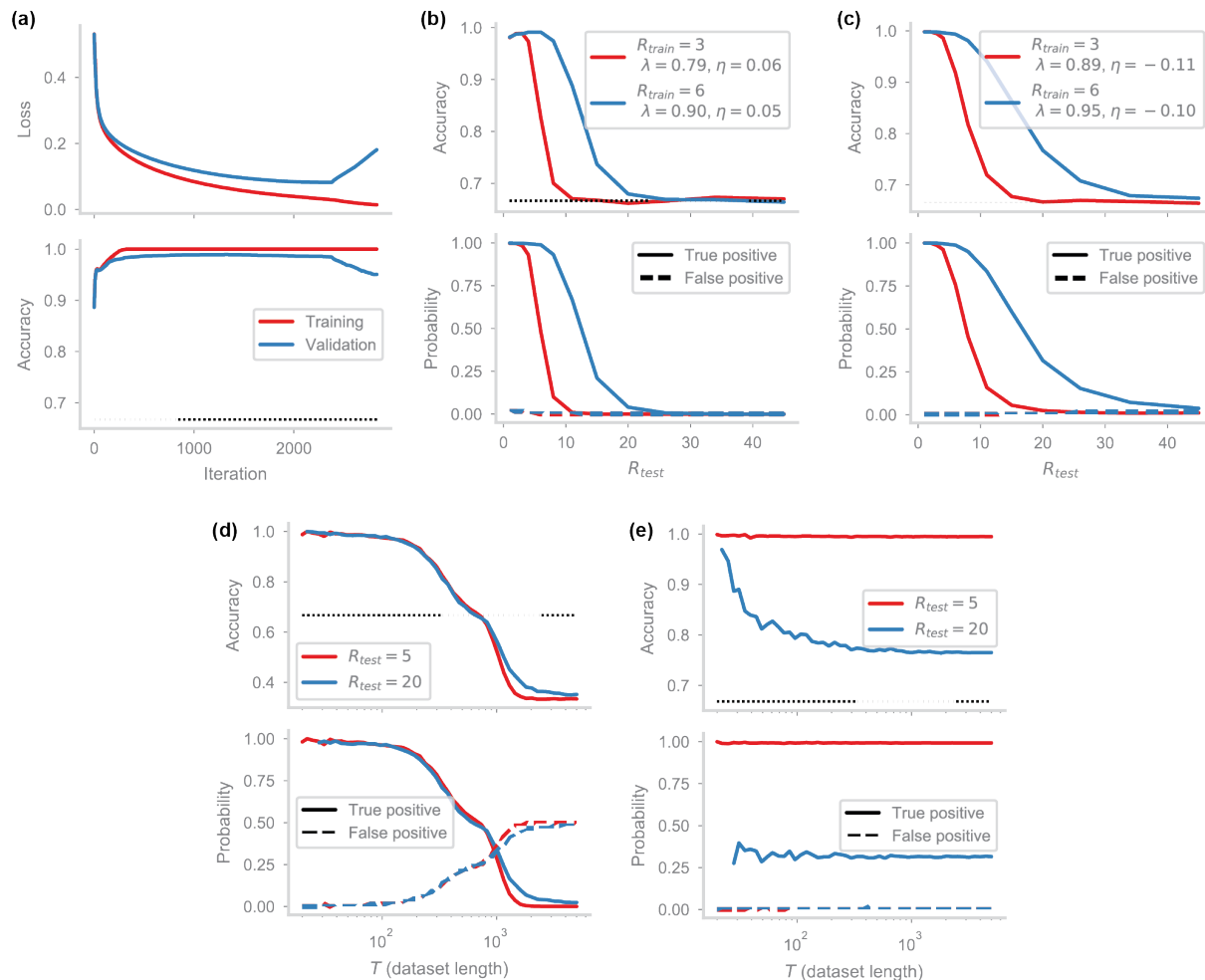
Figure 3. Hebbian vs. anti-Hebbian plasticity and continual operation. (a) Training the HebbFF network ( d = N = 100 ), as in Fig 2a. Both training and validation loss decrease, and accuracy increases, for a single instance of the dataset with R = 3 , indicating in-distribution generalization. Over many iterations, however, overtraining occurs due to the use of a single dataset, increasing the final validation loss. (b) HebbFF network trained with "infinite data" as in Fig 2b ( R = 3 , red; R = 6 , blue) shows not only in-distribution generalization to any dataset with R = 3 ( R = 6 , resp.), but also out-of-distribution to datasets with any smaller R 's. (c) HebbFF with a different initialization converges to a qualitatively different solution with a negative learning rate \eta , an anti-Hebbian learning rule, in contrast to the Hebbian solution in (b). The anti-Hebbian solution shows generalization performance over a larger range of R values than Hebbian. (d) Model from (Bogacz and Brown, 2003), evaluated on the continual familiarity detection task, varying the length T of the trial. Accuracy (top) is near-perfect regardless of the repeat interval R (blue vs. red curve) until the model reaches its capacity ( P^* \approx 100 for network size d = N = 100 ) because the model reliably stores the first P^* patterns. Accuracy rapidly drops below chance for T > P^* as the model begins to report familiar stimuli as novel (see Fig S2b). (e) HebbFF network operates continuously, as its accuracy (top) is consistent with the generalization curve from (c), with near-perfect performance for R_{test} = 5 and above 80% for R_{test} = 20 for any trial length. True and false probabilities (bottom) are better representations as accuracy (top) is artificially higher for small T due to the low proportion of familiar stimuli.
