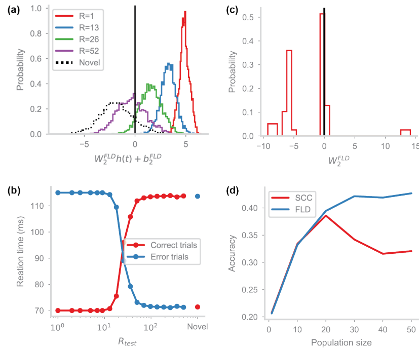
Figure S5. Behavior on augmented task. Panels correspond to the right-hand side plots of Fig 7(a-d), but for the classifier-augmented HebbFF network ( d = 25, N = 50 ) performing binary classification and familiarity detection simultaneously.
