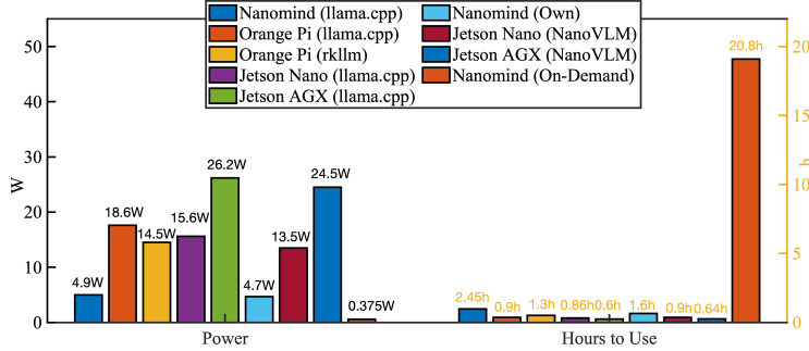
Figure 9: Power consumption (W) and estimated operating hours of NANOMIND when connected to a standard commercially available 2000 mAh power bank.
