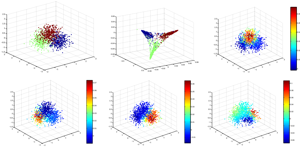
Fig. 15. Top, left to right: the dataset described in Example 8.4 with labels for each Gaussian random variable, the embedding given by the top 3 nontrivial eigenfunction of the graph Laplacian, the values of the scaling function \varphi_{6,1,1} . Bottom, left to right: values of the scaling functions \varphi_{6,1,2} , \varphi_{6,1,3} , and of the wavelet \psi_{8,5} .
