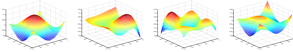
Fig. 14. Example of scaling functions at coarse level associated with a Beltrami diffusion on randomly distributed points on the unit square. For graphical reasons, we are plotting a smooth extension of these scaling functions on a uniform grid by cubic interpolation.
