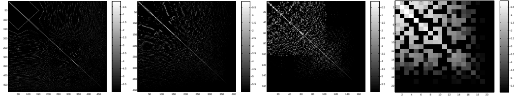
Fig. 12. The compressed powers of T at scale j = 1, 2, 5, 11 . The images are in logarithmic scale to show entries larger than 10^{-6} .
