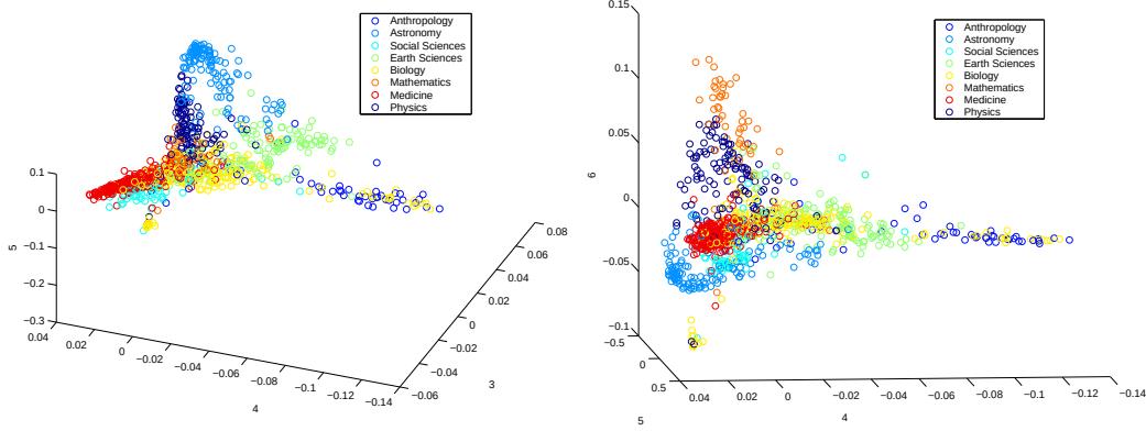
Fig. 5. Embedding \Xi_6^{(0)}(x) = (\xi_1(x), \dots, \xi_6(x)) : on the left coordinates 3, 4, 5, and on the right coordinates 4, 5, 6.
