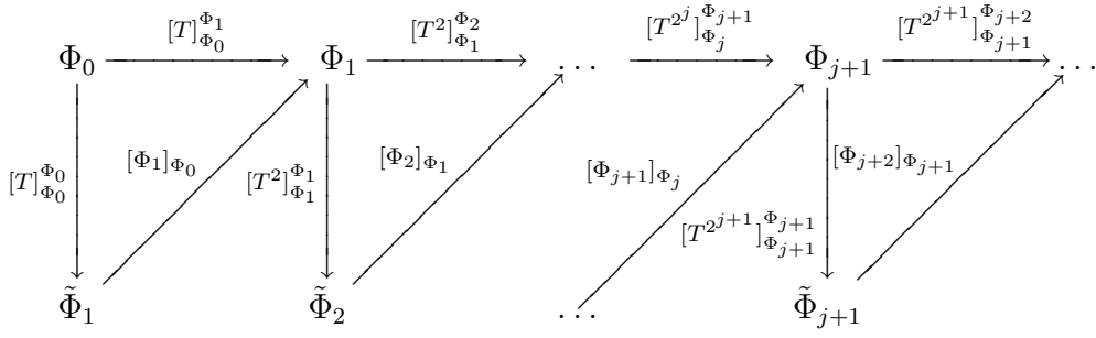
Fig. 8. Diagram for downsampling, orthogonalization and operator compression. (All triangles are commutative by construction)
