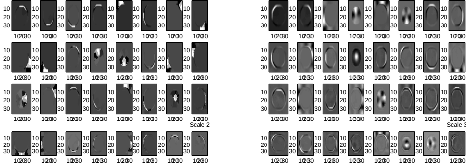
Fig. 17. Scaling functions at scale 2 and 3 on the graph of patches extracted from an image of a white full circle on black background, with noise.
