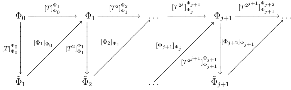
Fig. 2. Diagram for downsampling, orthogonalization and operator compression. (All triangles are commutative by construction)
