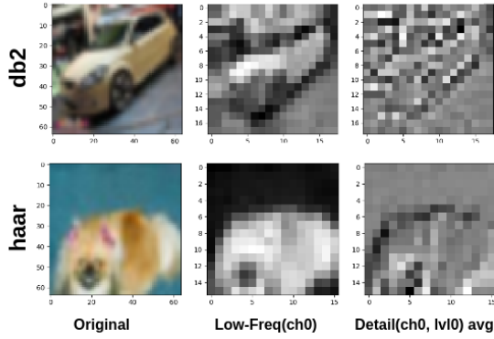
Figure 1. Wavelet-based decomposition and reconstruction. Left: Original images. Middle: Low-frequency subbands emphasizing global structure. Right: High-frequency details capturing fine textures.
