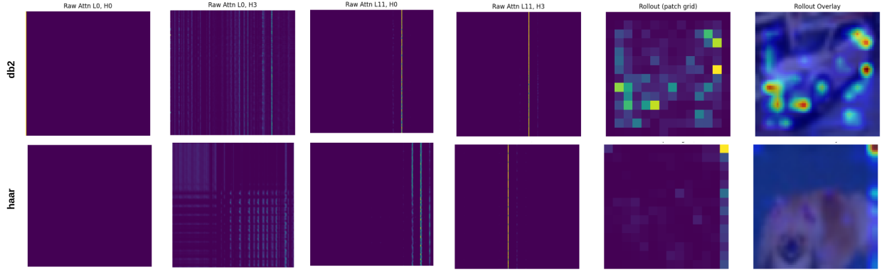
Figure 2. Comparison of ViT attention maps for Haar and DB2 wavelets. The first four columns represent raw attention from different layers and heads. The last two columns show attention rollout, with the final column overlaying attention on the original image. Haar wavelets exhibit higher sensitivity to high-frequency regions.
