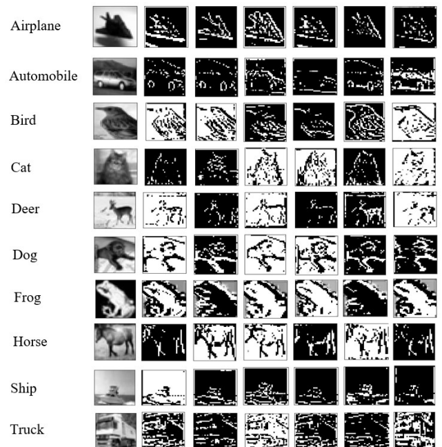
FIGURE 9. Gating units' activations (responses) for the first highway block in HWCC-19 trained on CIFAR-10 dataset. The first column shows the input images for the 10 different classes; other columns show units' activations for different convolution maps.
