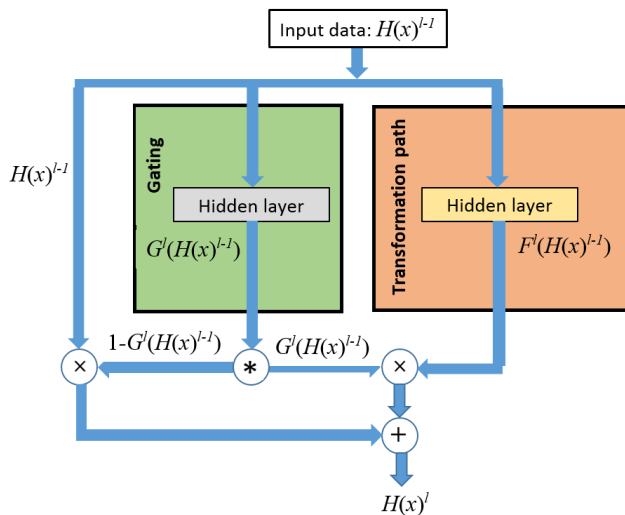
FIGURE 2. Highway network block [7].
