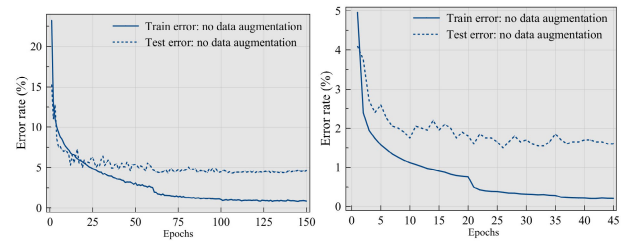
FIGURE 8. Error rate for HWCC-19. Left: Fashion-MNIST dataset. Right: SVHN dataset.
