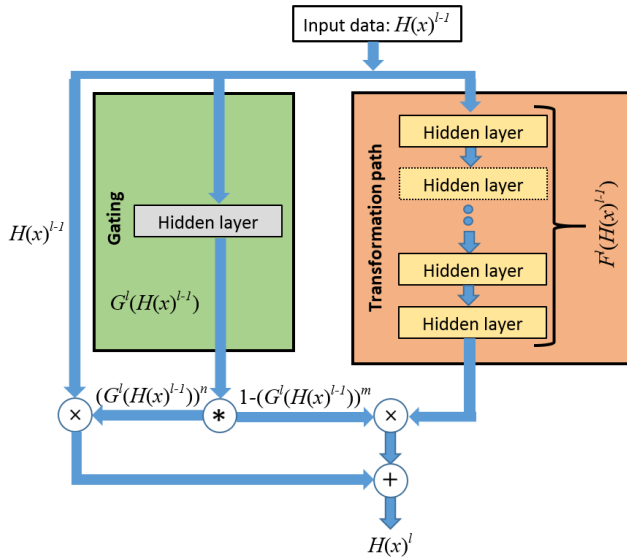
FIGURE 4. Highway network block with gate constraints (HWGC block) [19].
