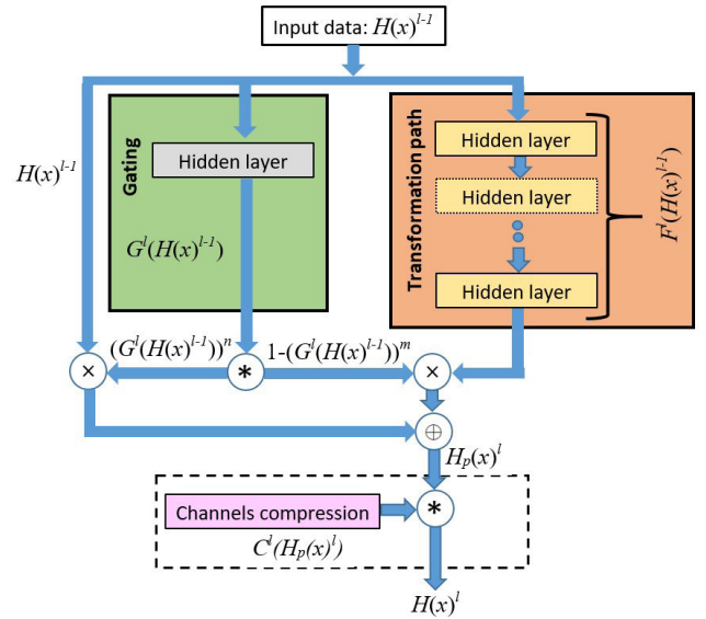
FIGURE 6. Proposed highway network block with gate constraints and concatenated features (HWCC block).
