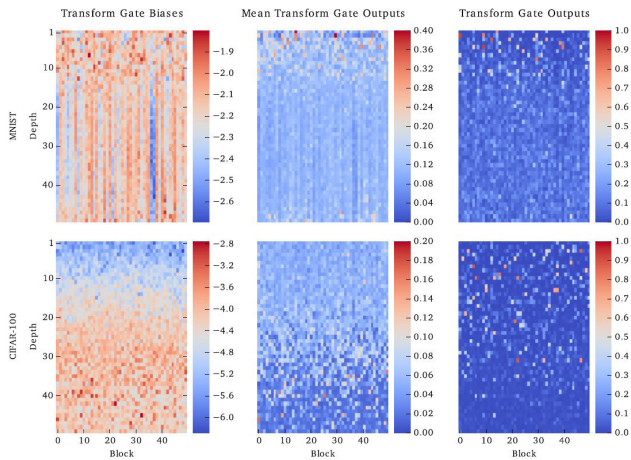
FIGURE 3. Original highway block learning attributes. Top row: 50-layer model trained on MNIST dataset. Bottom row: 50-layer model trained on CIFAR-100 dataset. First column: transform gate biases. Second column: mean of the transform gate outputs over the whole training set. Third column: transform gate output using a random training sample [7].
