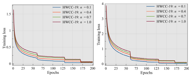
FIGURE 10. Convergence rate for HWCC-19. Left: CIFAR-10 dataset. Right: CIFAR-100 dataset.
