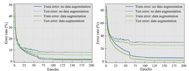
FIGURE 7. Error rate for HWCC-19. Left: CIFAR-10 dataset. Right: CIFAR-100 dataset.
