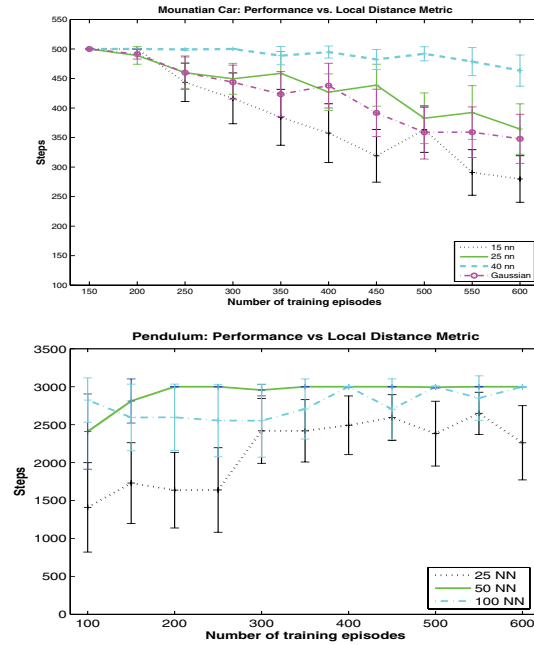
Figure 3: Performance on mountain car and inverted pendulum as a function of the nearest neighbors.
