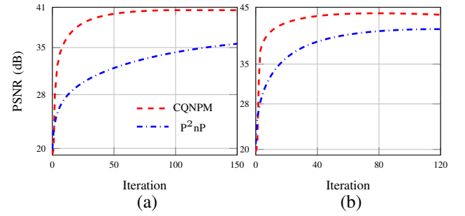
Fig. 12. Comparison of the preconditioned PnP ( P^2PnP ) method. (a) PSNR values versus iteration for spiral acquisition with the brain image; (b) PSNR values versus iteration for radial acquisition with the knee image.
