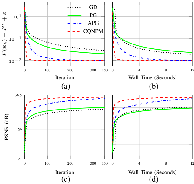
Fig. 8. Comparison of different methods with Cartesian acquisition on the brain image for \varepsilon = 9 \times 10^{-4} . (a), (b): cost values versus iteration and wall time; (c), (d): PSNR values versus iteration and wall time.
