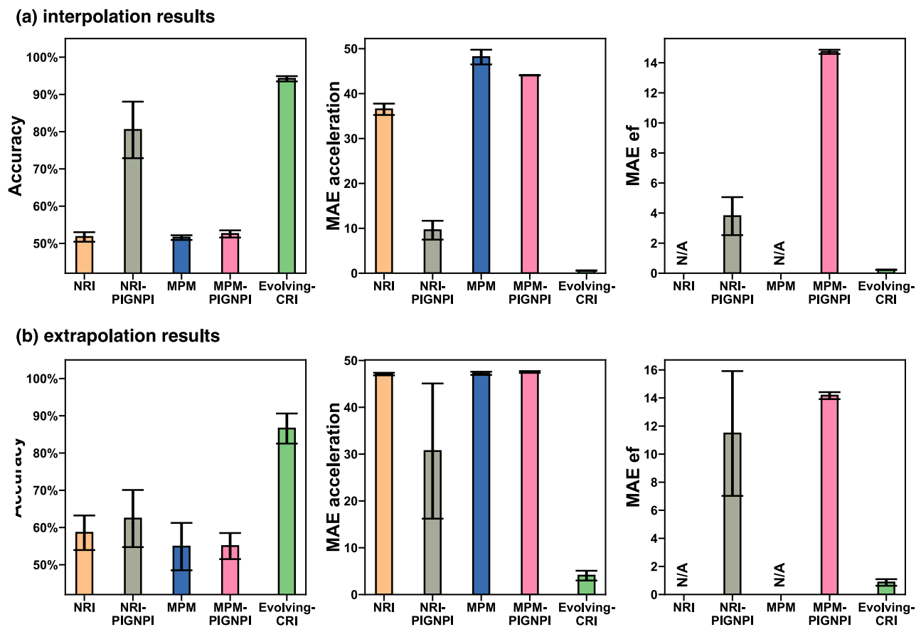
Fig. 6 | Performances of Evolving-CRI on the crystallization problem with an evolving graph topology. a Interpolation and b extrapolation results of Evolving-CRI and others. Mean and standard deviation are computed from five independent experiments. (left column of a, b ) Accuracy in inferring the interaction type. (center
