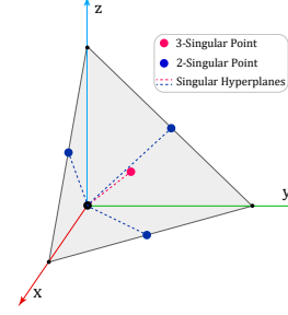
Figure 1. Singular Regions in a 3D One-Hot Setting.
