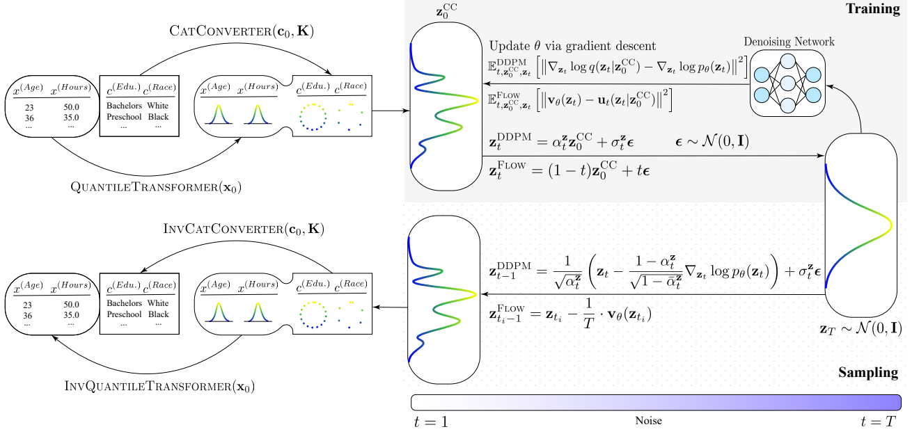
Figure 3. The TABREP Architecture. TABREP transforms and unifies the data space under a continuous regime via the our representation. A diffusion or flow matching process is trained to optimize the denoising network. Once training is completed, samples can be generated through a reverse denoising process before inverse transforming back into their original data representation.
