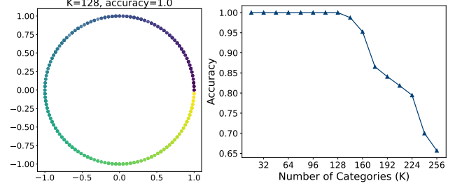
Figure 2. Separability of CatConverter. CatConverter preserves nominal representations for up to 128 categories.
