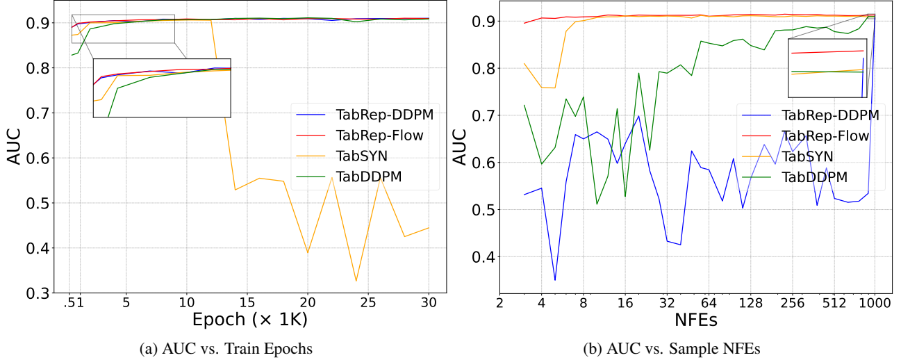
Figure 5. Training and Sampling Efficacy.
