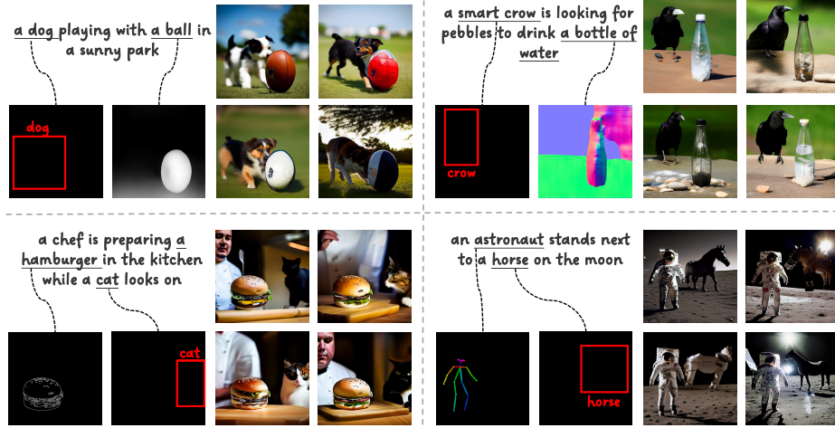
Fig. 5: Applications. Demonstrating scalability, our method adeptly manages complex scenes, seamlessly combining controller mechanisms like both ControlNet [45] and GLIGEN [20] simultaneously.
