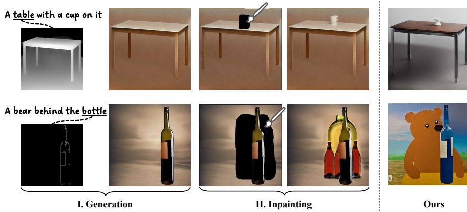
Fig.9: Left: Two-stage method. Right: Our Approach. Our method autonomously positions objects from the text in their correct locations, leveraging the generative model’s inherent priors, without the need for manual intervention such as masking. Inpainting is performed using [1].
