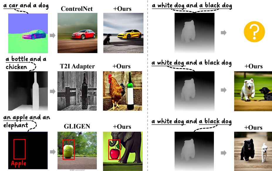
Fig. 2: Challenges in Multi-Condition Image Synthesis. Left: the “dominance” effect exists across various methods, where one object ( e.g. , car) overshadows the generation, omitting the other ( e.g. , dog). Right: The “ambiguity” issue, where it’s unclear which object from the text matches the intended depth condition.
