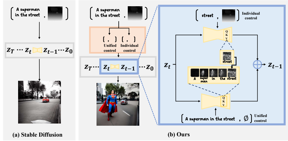
Fig.3: Image Synthesis using Text-Anchored Score Composition. Given a depth map of a street and a textual description specifying “a Superman in the street”, our method effectively generates the corresponding image.
