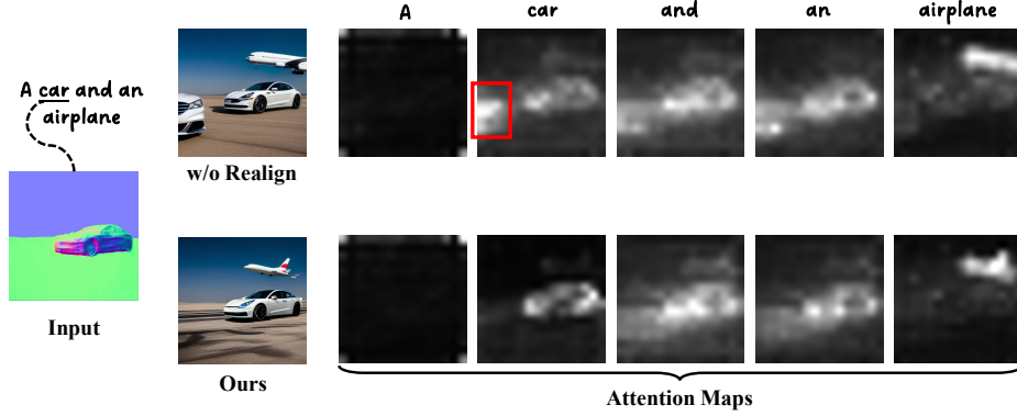
Fig. 4: Illustration of the “Attention Realignment” operation. The operation addresses mismatches between the unified score and individual scores during generation, preventing the final object from appearing multiple times, as individual score for the same token “car” will not contribute to the attention value in the red box.
