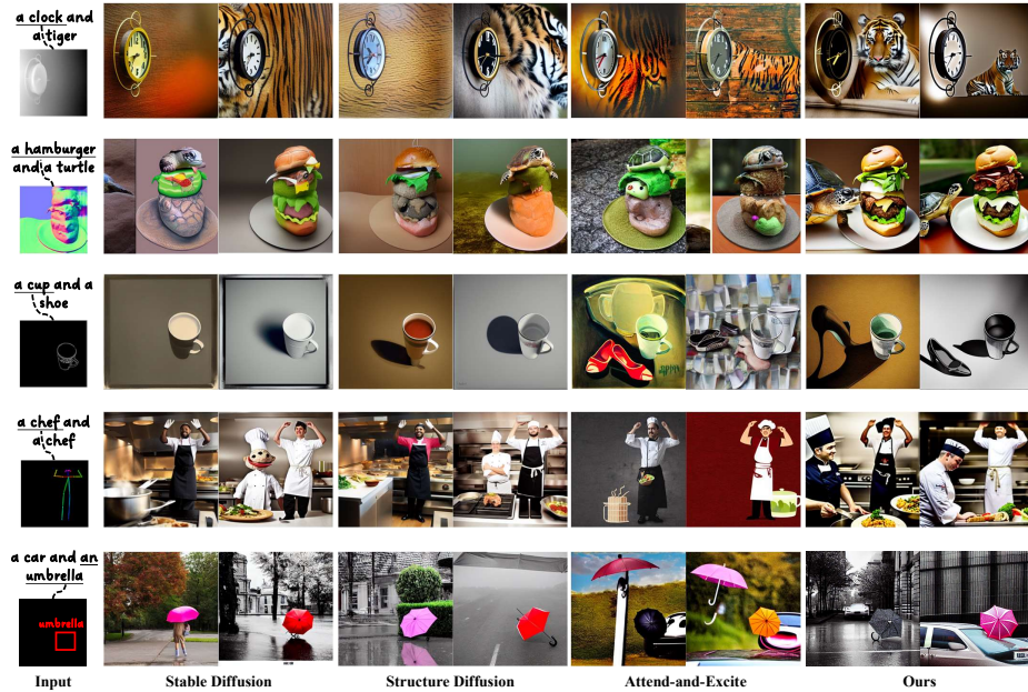
Fig. 6: Comparisons of “Dominance” Challenge. Our approach ensures that objects in the text, not linked to additional conditions, are still accurately generated ( e.g. , “tiger” in the first example).
