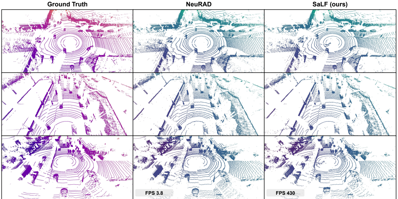
Figure 12. Additional qualitative comparison on LiDAR novel view synthesis.
