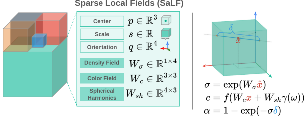
Figure 3. SaLF Representation. Left: SaLF models scenes using an adaptive sparse voxel grid with variable scales. Each voxel is characterized by static parameters and learnable parameters . Right: Within a voxel, for any point with normalized coordinates \mathbf{x} , the density \sigma and color c values are derived from W_\sigma and W_c along with the encoded view direction \gamma(\omega) modulating W_{sh} . The opacity \alpha of a ray is calculated using the density at the intersection midpoint and the traversal distance \delta .
