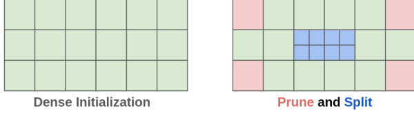
Figure 5. Initialization and Densification. SaLF initializes the scene representation with a coarse regular grid partitioning, then adaptively prune empty red while densifying blue regions that need fine-details.
