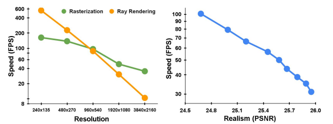
Figure 8. Efficiency analysis. Left: rendering speed comparison of rasterization vs. ray rendering across resolutions. Right: trade-off between rendering speed and realism.
