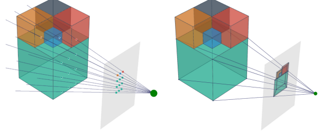
Figure 4. SaLF can be efficiently rendered by ray-casting (left) and rasterization (right). Ray casting is more flexible and can handle more complex physics phenomena, while rasterization is more efficient for pinhole cameras. Both follow the same rendering equation.
