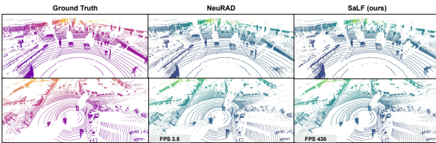
Figure 7. Qualitative comparison on LiDAR novel view synthesis. Our method achieves comparable LiDAR rendering performance compared to NeuRAD, while being 100\times faster in rendering.
