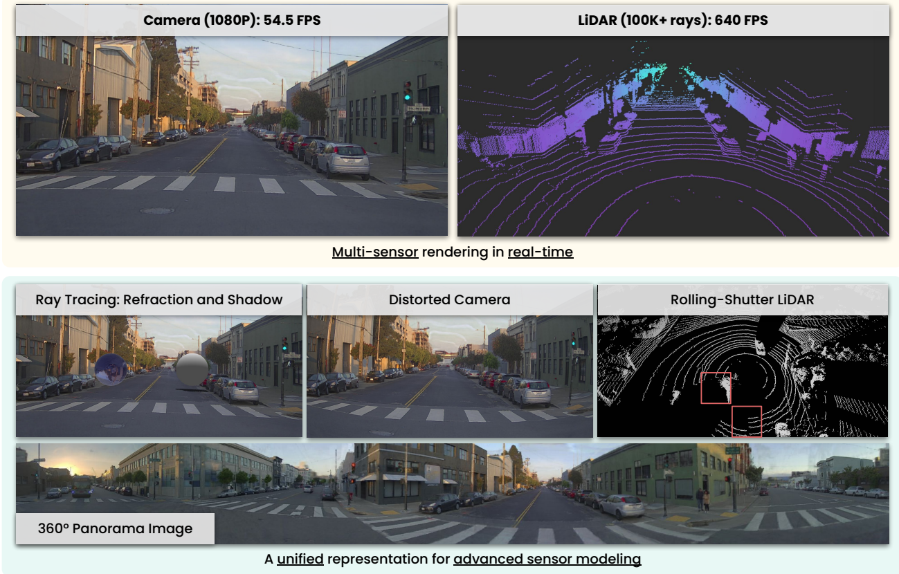
Figure 2. Real-time self-driving sensor simulation with SaLF representation. Our method achieves high-performance rendering for both camera and LiDAR, and supports advanced features including secondary effects ( e.g. , refraction, reflection and shadow) and complex sensor models ( e.g. , fisheye, rolling-shutter and panoramic cameras). This is made possible by an efficient and unified representation that supports both rasterization and ray-tracing.
