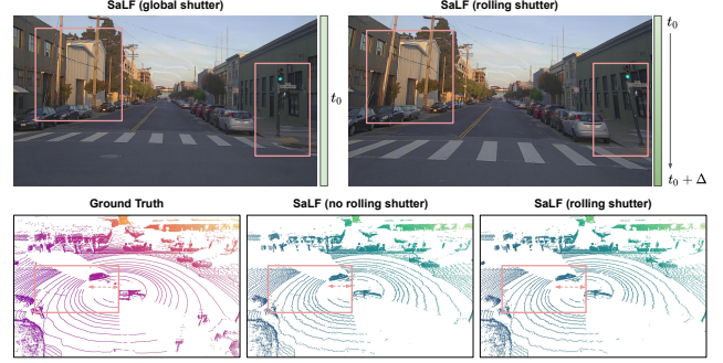
Figure 10. Rolling-shutter simulation via efficient ray-based rendering. Top: We render the same view using global shutter and rolling-shutter camera models (see highlighted distorted region). Bottom: SaLF simulates rolling-shutter effect and accurately match ground truth point clouds (see lidar sweep seam and relative position for the dynamic actor in the highlighted region.)
