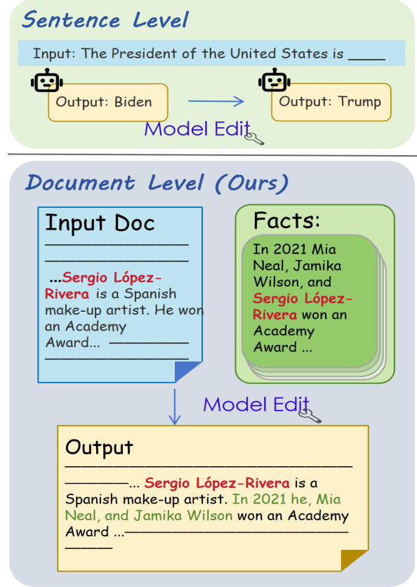
Figure 1: An example of DocMEdit. The input and output of DocMEdit are both document-level contents. Model editing should inject multiple facts to be edited into the model, enabling the edited model to output the updated document.
