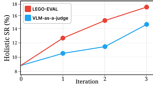
Figure 7: Comparison of refinement results using VLM-as-a-judge and LEGO-EVAL as feedback signal.
