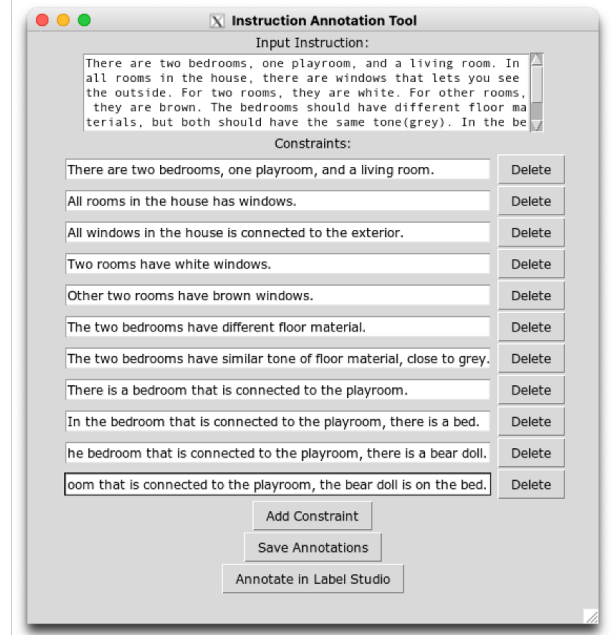
Figure 8: Our annotation tool used for annotating constraints.
