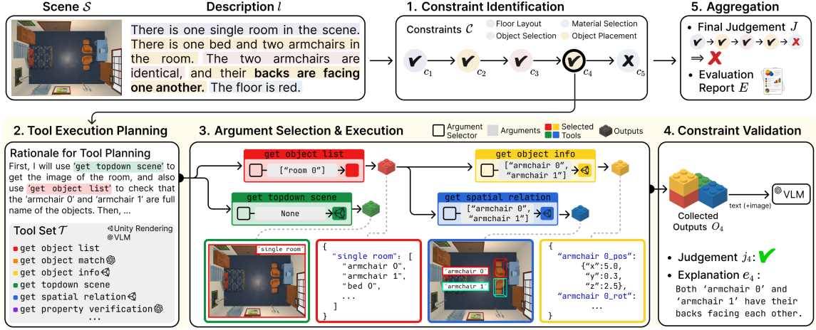
Figure 4: LEGO-EVAL. All steps are performed by a VLM judge \mathcal{M} , which plans tool execution, selects arguments, executes tools, evaluates each constraint, and aggregates the results into a final judgment J and a report E .
