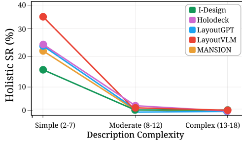
Figure 6: Description complexity vs. Holistic SR.
