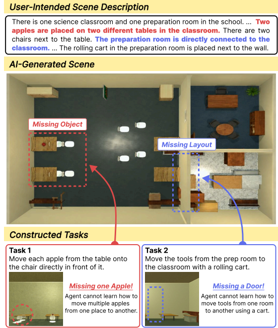
Figure 1: An example of misalignment in text-guided 3D scene synthesis. The generated scene spawns only one of two apples and omits the door, making the constructed tasks unexecutable and unlearnable.
