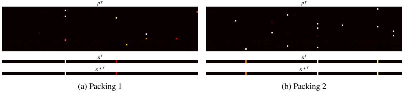
Figure 4. Examples of generated projection matrix \mathbf{P}^\top using our method (top), solution \mathbf{x}^\top obtained with our method (middle), and solution \mathbf{x}^{*\top} obtained by solving the original LPs without dimensionality reduction (bottom) for two different packing problems. Black represents zero, which is the lowest value. The horizontal axis in all plots represents the variables, and the vertical axis in \mathbf{P}^\top corresponds to the reduced variables. 150 variables out of 500 and 30 reduced variables out of 50 are shown for better visibility. The same model with K = 50 was used to obtain \mathbf{P} and \mathbf{x} in these two problems.
