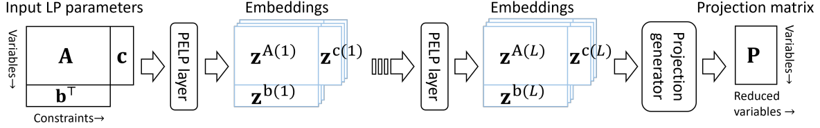
Figure 2. Our model takes LP parameters as input, and outputs a projection matrix.
