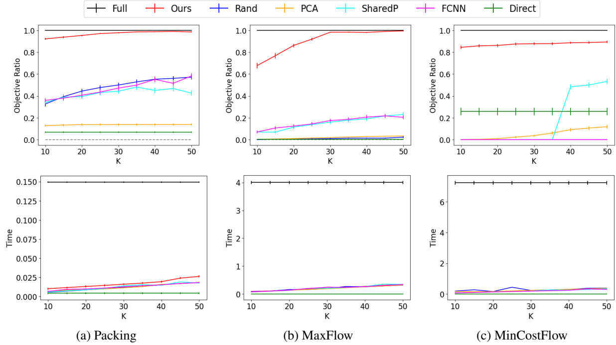
Figure 3. Average test objective ratio (upper row) and computational time in seconds for solving an LP (lower row) with different reduced dimensions K . Bars show the standard error.
