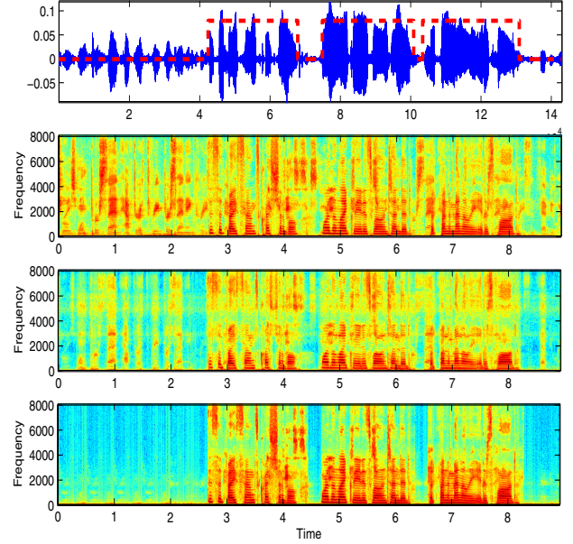
Figure 2: Enhancement Results (sequentially from top to bottom): a) the original bone sensor data; b) spectrogram of noisy utterance; c) result of the DF algorithm; d) result of the proposed model.
