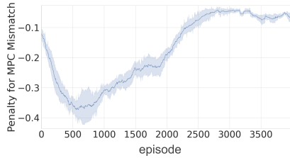
Fig. 6: The figure shows the penalty given to the agent for deviating from the MPC safe actions. The bold lines show the average while the shaded area show the standard deviation over three different random seeds. The penalty decreases through the training indicating that the agent learns to match the MPC safe actions.
