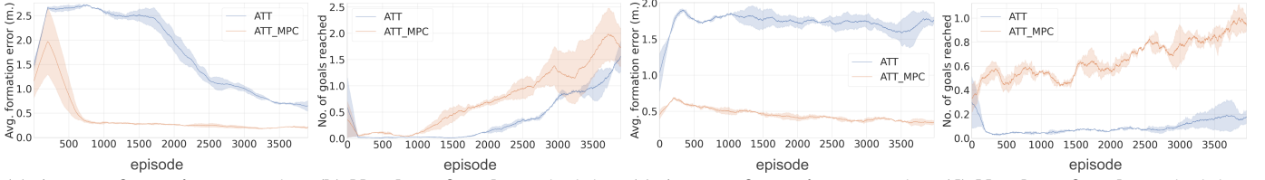
(a) Average formation error during the first environment. (b) Number of goals reached during the first environment. (c) Average formation error during the second environment. (d) Number of goals reached during the second environment.
