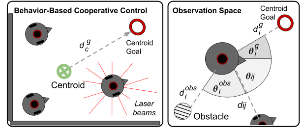
Fig. 2: The observation space per robot includes lidar readings (red lines), distances and headings to the goal ( d_i^g , \theta_i^g ), two neighbors ( d_{ij} , \theta_{ij} ), and the closest obstacle ( d_i^{obs} , \theta_i^{obs} ). Additionally, robots have information about the centroid's distance to the goal ( d_c^g ).
