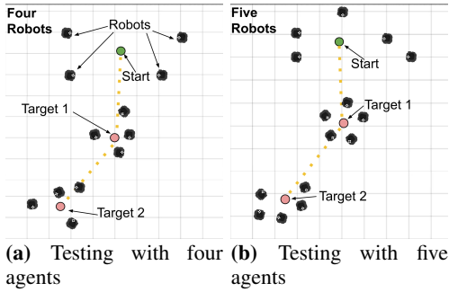
Fig. 8: Example scenarios (a) and (b) show the generalization of the trained policy to a larger team of robots. The robots successfully move their centroid from the starting location (green circle) to the target location (red circle). The yellow lines indicate the movement of the centroid through the different locations.
