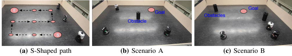
Fig. 7: The figures show the S-Shaped path tests and two scenarios of the obstacle avoidance tests. (a) shows the S-shaped path. The red circles indicate the target locations for the centroid of the formation, where the first and final targets are indicated by the letters S, E, respectively. (b,c) show two different scenarios for obstacle avoidance. The robots start from the shown configurations and navigate towards the goal while avoiding collisions with the obstacles shown in the figures.
