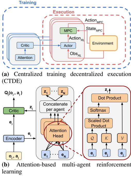
Fig. 3: Illustrations of the CTDE architecture and attention module. (a) At each time step, the agent interacts with the environment to receive the current observation Obs_{RL} , including relative information about the two neighbors and the closest obstacle, and outputs the Action_{RL} . The MPC controller receives the State_{MPC} , overrides any unsafe actions to prevent collisions, and sends Action_{MPC} to the robot. During training (blue dashed), critics share all agents' observations, while during execution (red dashed), each actor accesses only its own observation. (b) In the attention-based critics, observations are encoded separately and fed into attention heads to calculate weights based on the query, and the key-value pairs. The attention output is then concatenated with the states and fed into the critics.
