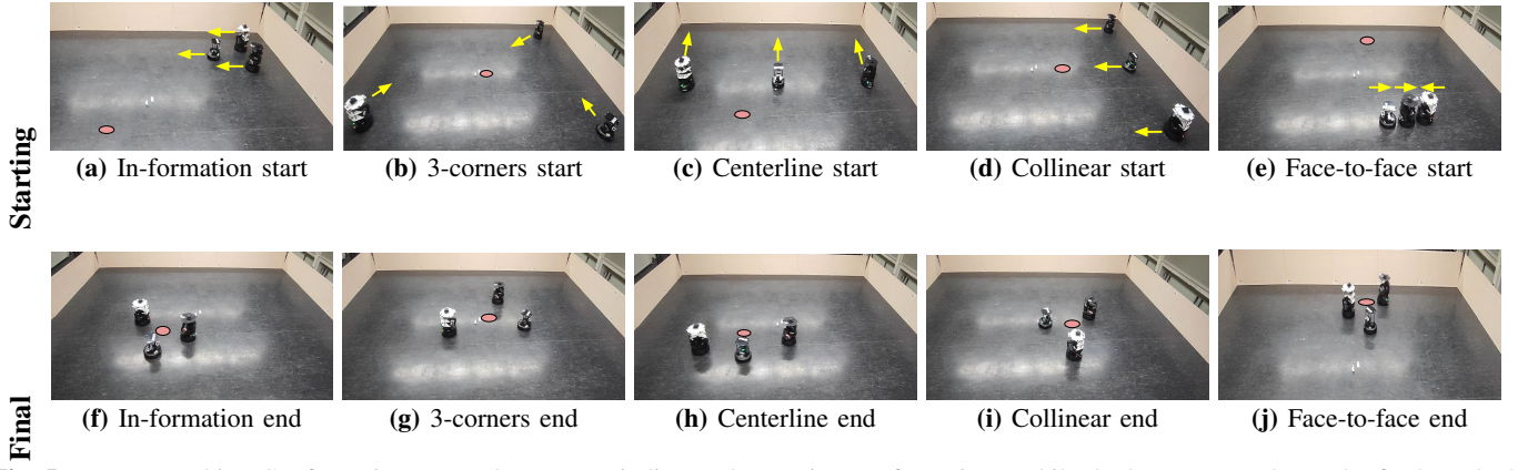
Fig. 5: Target Reaching Configurations test. The top row indicates the starting configurations, while the bottom row shows the final reached configurations by our approach. The yellow arrows indicate the starting orientation of the robots, while the red circles show the target location for the centroid of the formation. The configurations are arranged from left to right in terms of difficulty. The Collinear and Facing each other configurations were not experienced during the training, making them more difficult compared to the other configurations. However, our approach was able to successfully complete the tasks with zero collisions.
