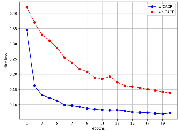
Figure 6. During training, the Dice loss with the CACP configuration converges faster compared to the process without the CACP configuration.
