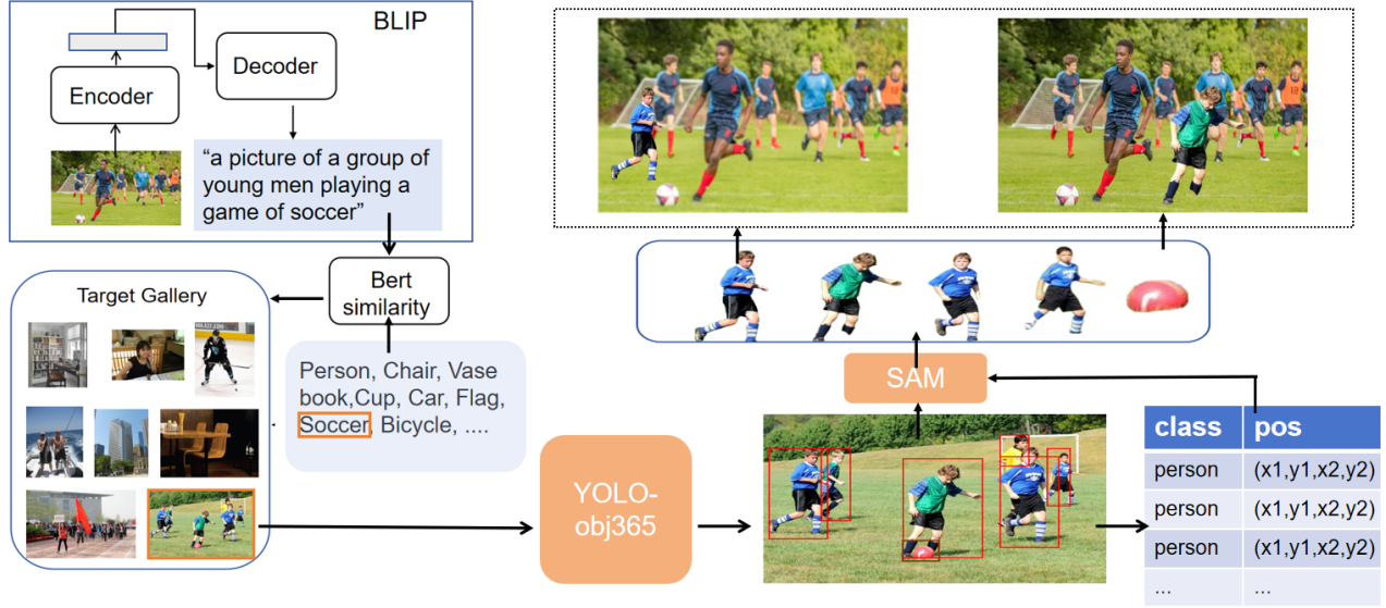
Figure 2. Our method’s pipeline involves leveraging BLIP and BERT to select the best-matched target image from a gallery. Subsequently, the corresponding mask is obtained using YOLO and SAM. A single base-target pair can generate multiple augmented images based on user preferences.
