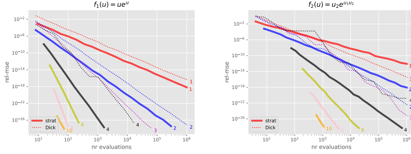
Figure 2: Relative MSE (mean squared error) vs number of evaluations for the vanishing estimator (thick lines) and Dick's estimator (dotted line). The value of r (stratified) or \alpha (Dick's) are printed next to each curve. Left: f_1 ; Right: f_2 .
