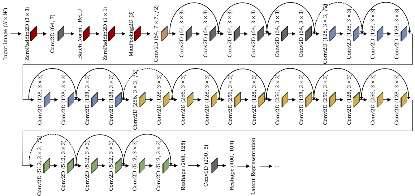
FIGURE 13: Offline HWR method based on the ResNet34 architecture [120].
