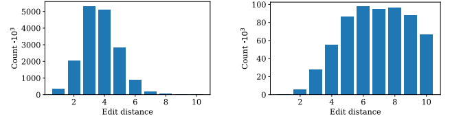
(a) OnHW-words500.
