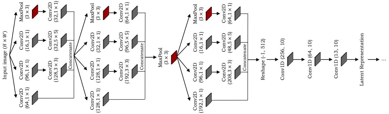
FIGURE 12: Offline HWR method based on Inception modules [119].
