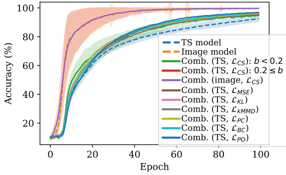
FIGURE 8: Accuracy of single- and cross-modal representation learning over all epochs.
