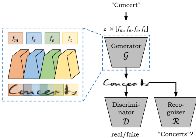
FIGURE 5: ScrabbleGAN concept by [40] of generating the word “Concerts”.
