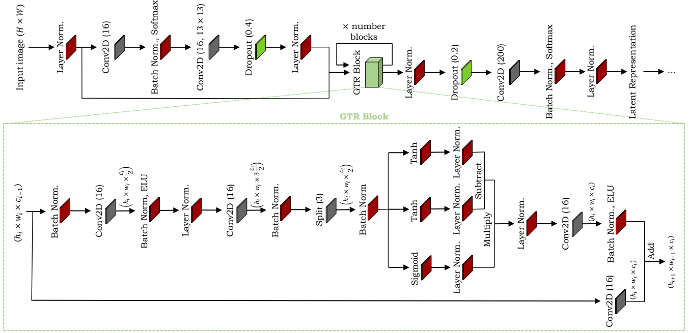
FIGURE 14: Offline HWR method based on the gated text recognizer architecture [73].
