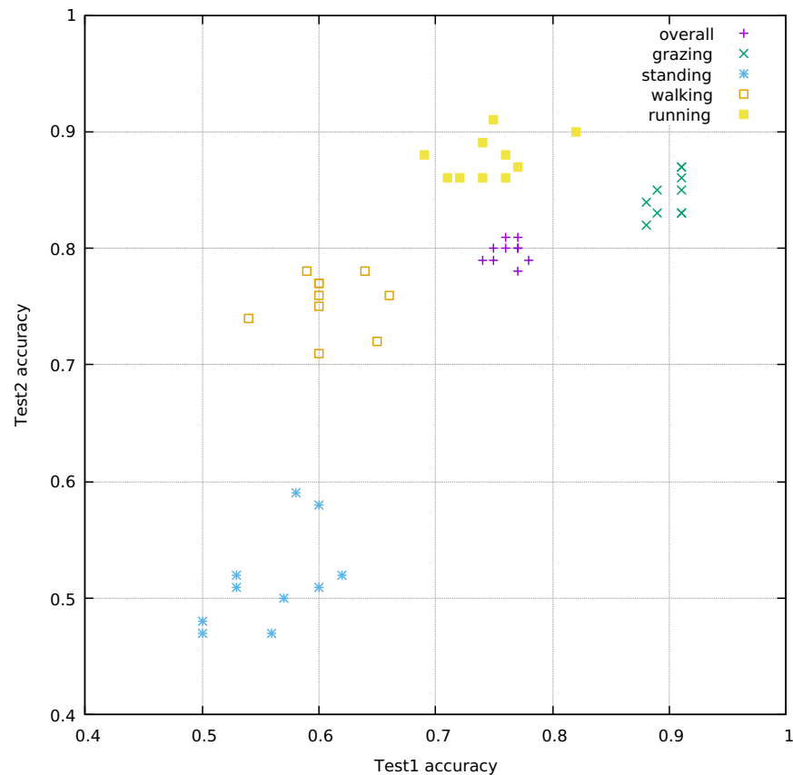
Figure 7: Cross-correlation of network performance on Test set 1 and Test set 2 for the whole dataset as well as for each behavior class.
