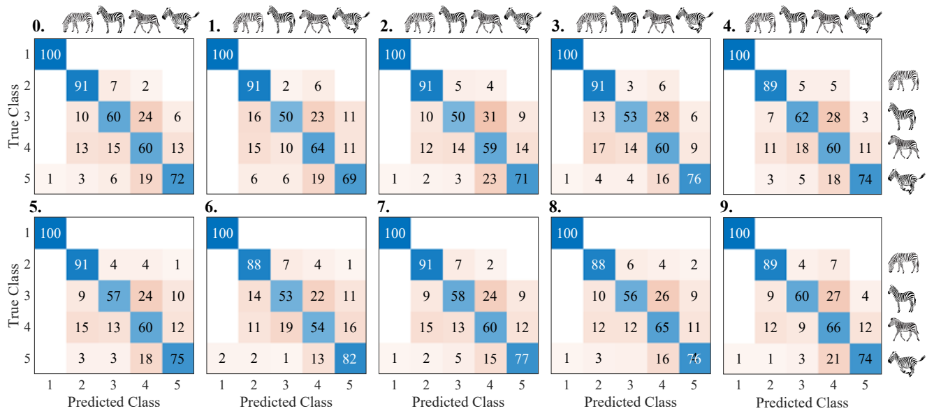
Figure 3: Groundtruth vs. Detection Confusion matrix for 10 trained networks - Test set 1. Each row shows the percentage of detections (per column) for each ground truth class in the order: “unknown”, “grazing”, “standing”, “walking”, “running”.
