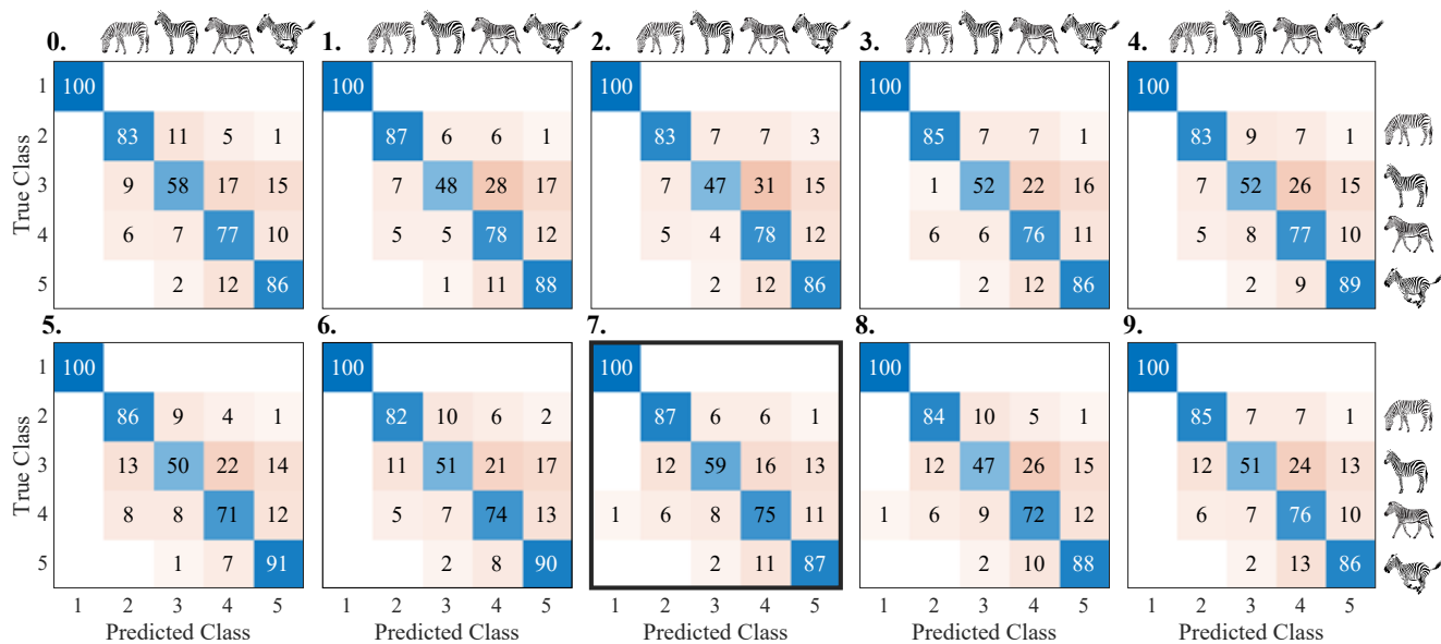
Figure 4: Groundtruth vs. Detection Confusion matrix for 10 trained networks - Test set 2. Each row shows the percentage of detections (per column) for each ground truth class in the order: "unknown", "grazing", "standing", "walking", "running". The confusion matrix for the best performing network (network 7) is highlighted with a bold boundary.
