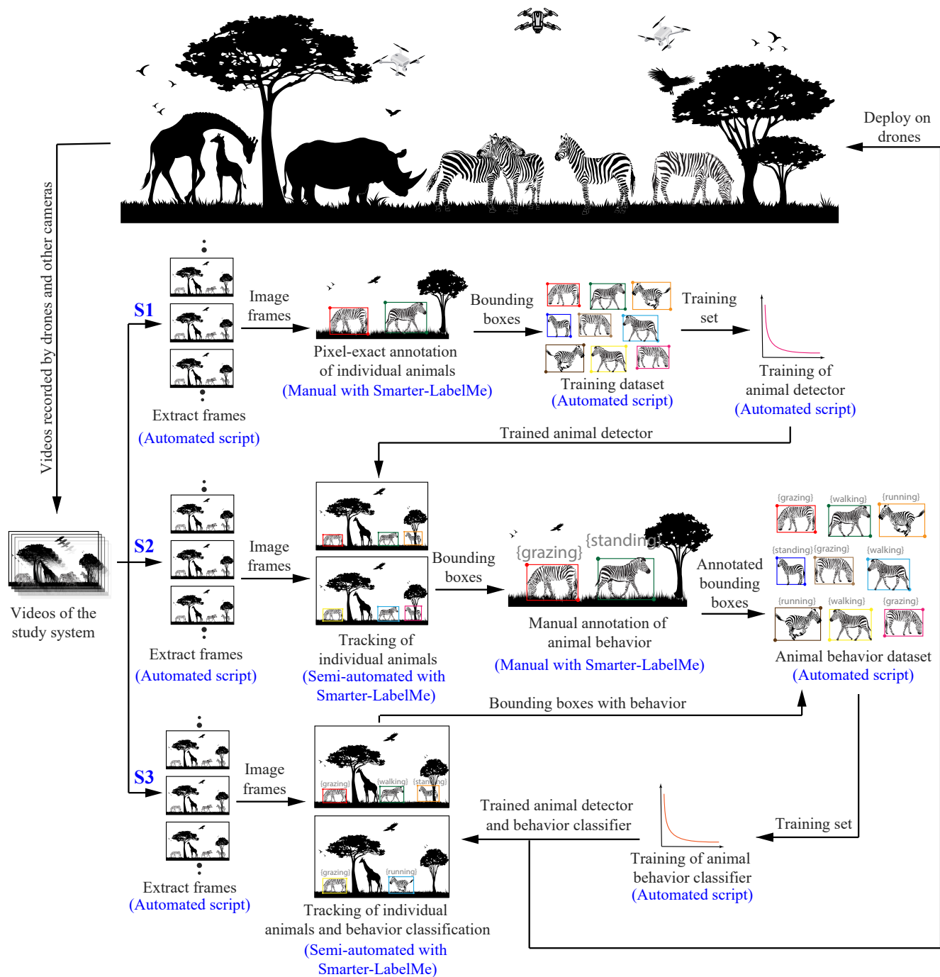
Figure 2: Architecture of the semi-automated animal detection and behavior inference workflow. The workflow is divided into three streams - S1, S2, and S3. The workflow is initiated from S1 by manually annotating pixel-exact bounding boxes of animals to generate animal detector training data followed by training the detector network [18]. The trained animal detector is used in S2 to perform manual annotation of behaviors and generate a training dataset to train the behavior classifier. S3 takes the output of S2 to semi-automate the entire behavior annotation process and rapidly generate more training data to fine-tune the behavior classifier and reach sufficient animal detection and behavior inference accuracy for deployment in field missions.
