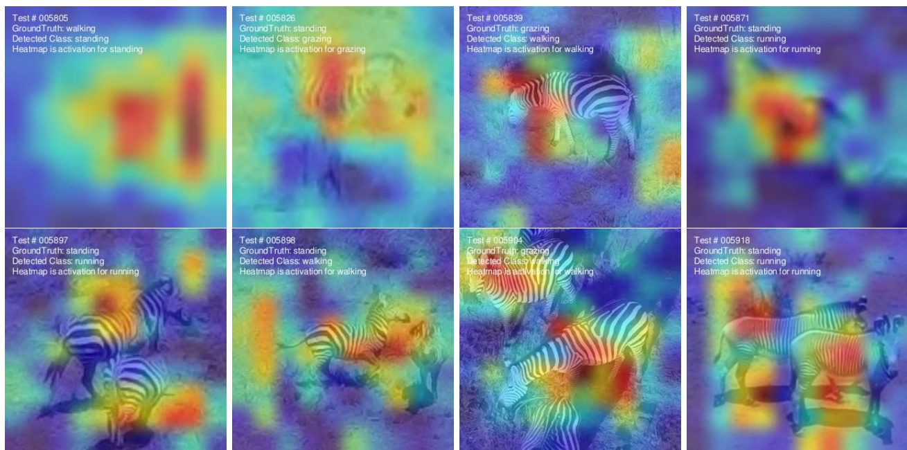
Figure 6: Class Activation Heatmaps (CAM) for failure cases. Prominent failures happen when the zebra is very distant and hard to distinguish, but also when there are multiple zebras in close proximity, confusing the classifier with conflicting information. Steep viewing angles and simultaneous actions (grazing while walking) also seem to sometimes confuse the network.
