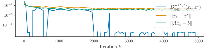
Figure 1: When R + F is not strongly convex, the Bregman divergence alone is not enough to provide useful convergence rates as it may not be point separating. Here for R = \|\cdot\|_1 , F = 0 , D_R^{-A^*y^*}(x_k, x^*) vanishes quickly, while the iterates x_k of (12) are still far from their limit x^* (synthetic noiseless data, exact prox).
