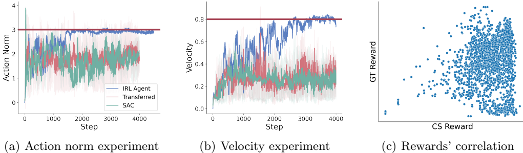
Figure 2: Single task cs-reward : In (a), (b), we plot the rewards during the IRL process (IRL Agent), an RL agent with the learned cs-reward from the IRL process (Transferred), and a baseline RL agent without any common sense component (SAC). The red horizontal line represents the target value in velocity/action norm see Eq. 10 and 11. The scatter plot (c) shows the correlation between the ground-truth reward and the learned CS-Reward.
