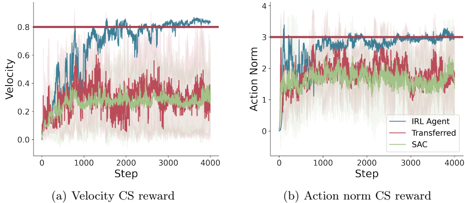
Figure 5: Single task cs-reward : Visualization of the rewards during the IRL process (IRL Agent), an RL agent with the learned cs-reward from the IRL process (Transferred), and a baseline RL agent without any common sense component (SAC). The red horizontal line represents the target value in the ground truth reward, see Eq. 10 and 11. This experiment was conducted on the coffee-button setup task.
