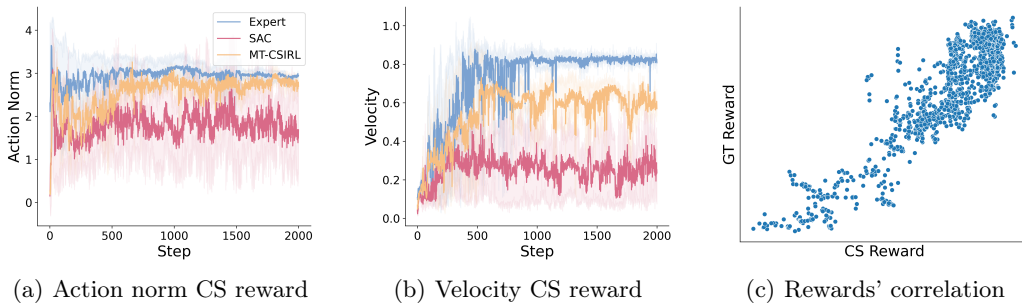
Figure 3: Ground Truth CS-Reward : In (a) and (b), We show the ground-truth common sense behavior on three different experiments. Expert: maximizes task reward and ground-truth cs-reward. MT-CSIRL: trained with the learned cs-reward and with the task reward. SAC: "vanilla" training, trained only with task reward. In (c) we visualized the scatter plot between Ground-Truth & Learned CS-Reward from MT-CSIRL method, on Velocity Experiment.
