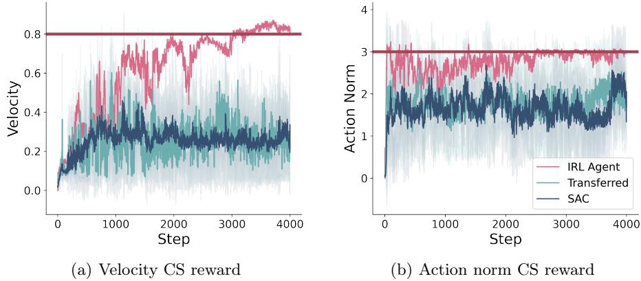
Figure 4: Single task cs-reward : Visualization of the rewards during the IRL process (IRL Agent), an RL agent with the learned cs-reward from the IRL process (Transferred), and a baseline RL agent without any common sense component (SAC). The red horizontal line represents the target value in the ground truth reward, see Eq. 10 and 11. This experiment was conducted on the button-press-topdown-wall setup task.
