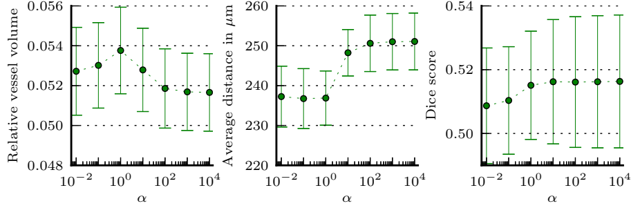
Figure 6: Sensitivity study on the weight parameter \alpha performed on two \mu\text{MRA} datasets. The parameter \alpha has a limited impact with respect to the depicted scores. Averages are within 5.16 % and 5.37 % for relative vessel volume, 236 \mu\text{m} and 251 \mu\text{m} average distance and 50.8 % and 51.6 % Dice (cf. Fig. 8).
