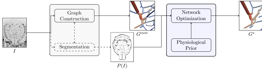
Figure 1: Workflow: In a first stage (gray box), the image volume I is processed so as to obtain an overconnected graph G^{\text{over}} as well as a confidence measure for vessels such as the confidence map P(I) . In the following step, the network G^* is extracted from G^{\text{over}} in a optimization that considers both image evidence (according to P(I) ) and geometric-physiological prior knowledge. In this paper, we focus on the network optimization step (blue), where both image evidence and geometrical relationships of certain network motifs, namely continuing pairs and bifurcations are considered.
