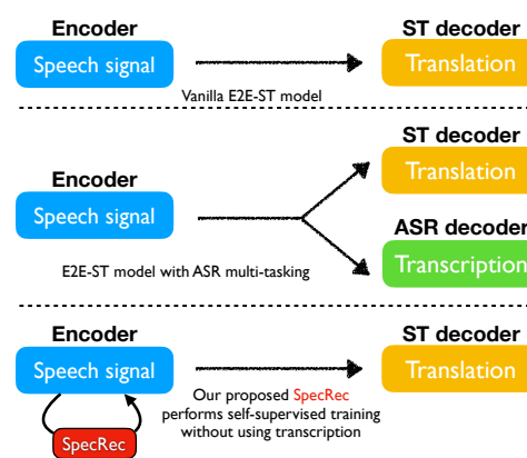
Figure 1: Comparisons with different existing solutions and our proposed Spectrogram Reconstruction (SpecRec).
