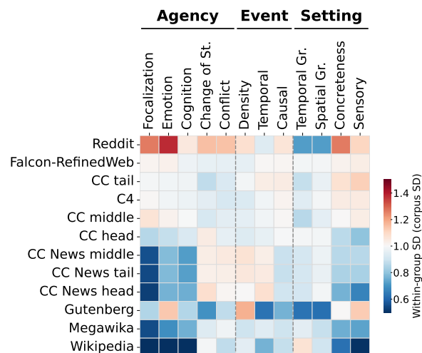
Figure A14: SD of z -scored narrative features by source , ordered by hierarchical clustering on profile similarity.
