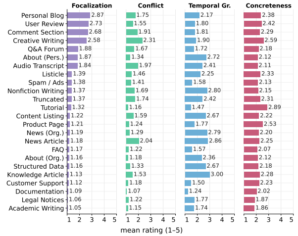
Figure 9: Bar plot of the focalization, conflict, temporal grounding and concreteness feature scores by format . All features are shown in App. B.1.
