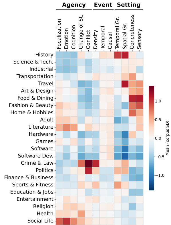
Figure A12: Mean z-scored narrative features by topic , ordered by hierarchical clustering on profile similarity.
