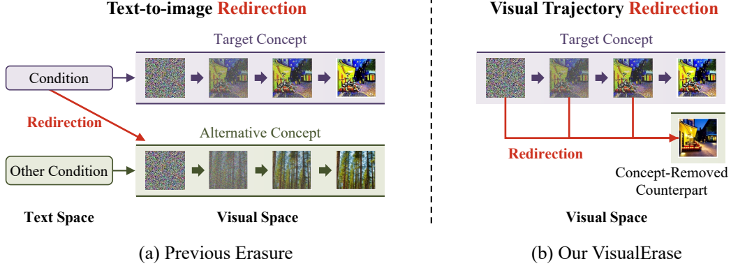
Figure 1: Conceptual comparison of text-to-image redirection and visual trajectory redirection. (a) Text-to-image redirection steers generation under a target text condition toward an alternative concept, but does not necessarily remove the underlying ability to generate the target concept. (b) VISUALERASE instead supervises denoising from source visual states at different timesteps toward a content-aligned, concept-removed counterpart that defines the desired visual endpoint. Red arrows indicate the respective redirection objectives.
