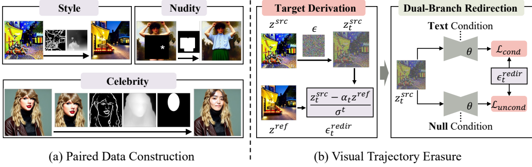
Figure 2: Overview of VISUALERASE. (a) Paired Data Construction creates a content-aligned counterpart in which the target concept is absent. (b) For visual trajectory erasure, Target Derivation converts the pair into a denoising target, which Dual-Branch Redirection applies under both the source and empty text conditions. Counterpart Retention is described in the text.
