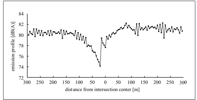
Figure 4. Noise emission profile L_{W,s} for the inbound (left) and outbound (right) lane of the major arm of the priority-to-the-right intersection ( D_M = D_m = 100 \text{ vehicles}\cdot\text{h}^{-1} , F = 5 \% , R = 40 \% ), averaged over 5 simulation runs.
