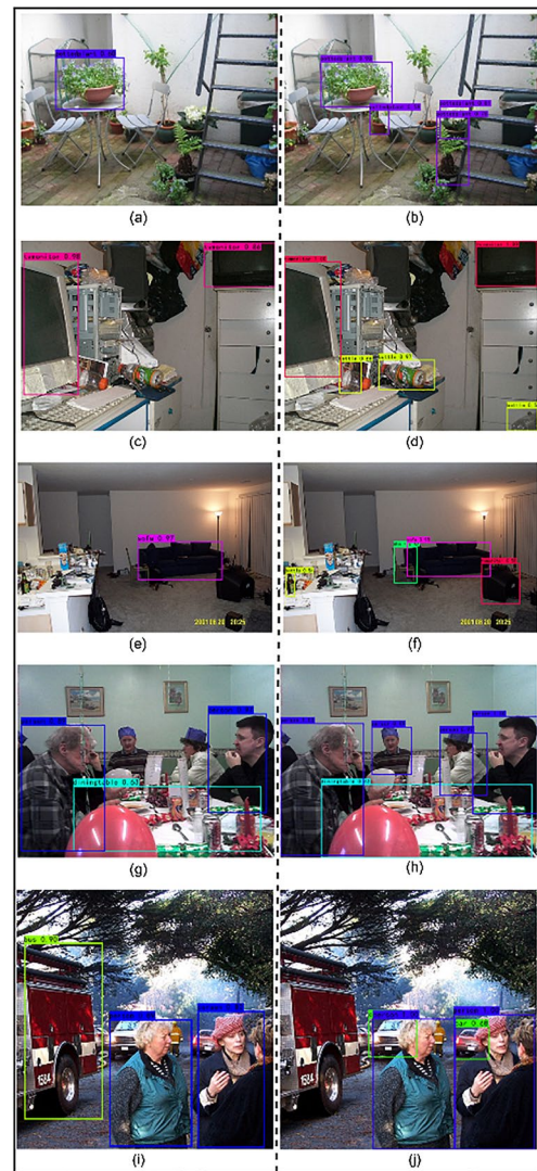
Fig. 7 The images in the left column are the results of the base SSD, and the images on the right are the test results of our method
