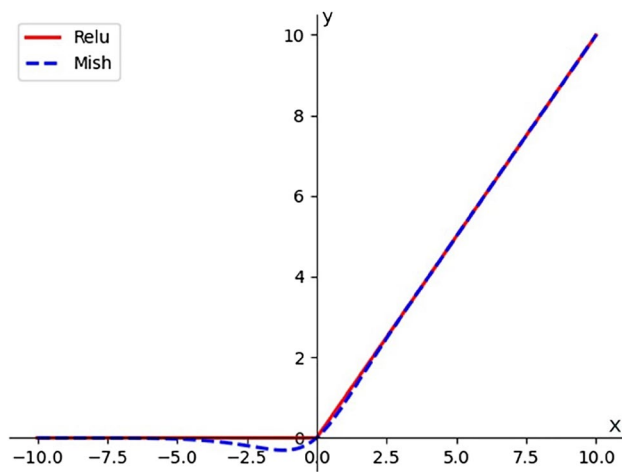
Fig. 6 Mish function and ReLU function images
