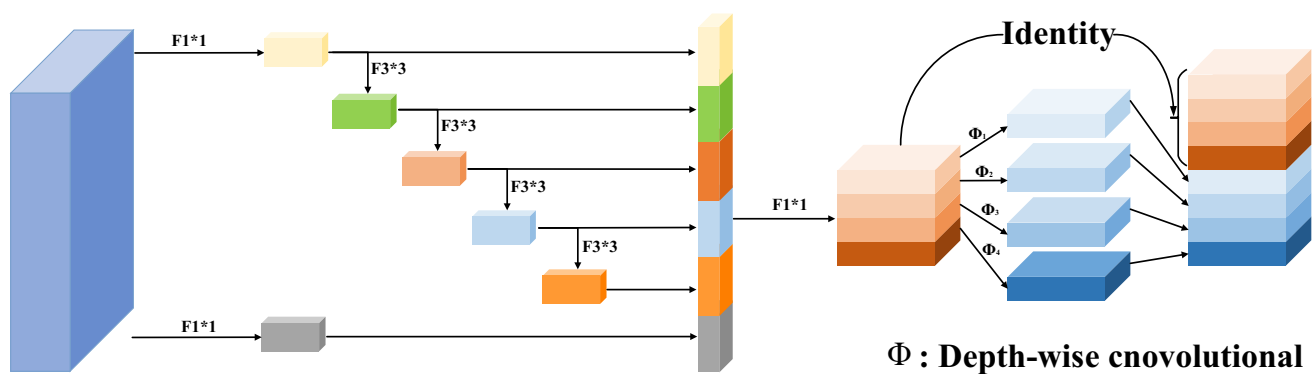
Fig. 5 FCR block
