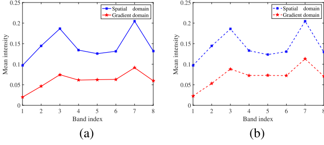
Fig. 3. Mean intensity on the spatial and the gradient domains for (a) the GT (reference) image and (b) the corresponding LRMS image on the simulated Rio WorldView-3 dataset.
