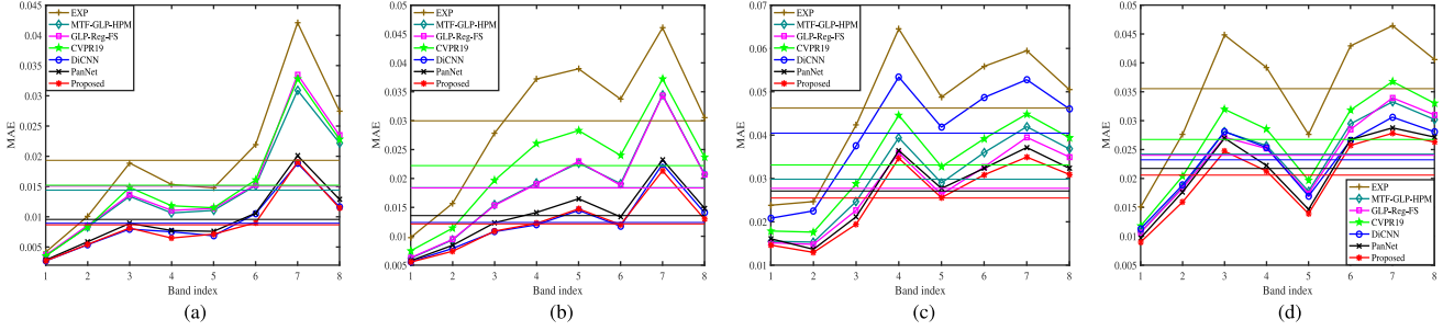
Fig. 6. Spectral MAE curves for all the methods on the reduced resolution (simulated) datasets: (a) Rio dataset, (b) Tripoli dataset, (c) WashingtonDC dataset, and (d) Stockholm dataset. The horizontal lines represent the average value of the MAEs calculated for all the spectral bands. The lower the value, the better the performance.
