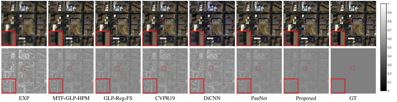
Fig. 5. Fusion results on the reduced resolution (simulated) WashingtonDC dataset (source: WorldView-2). Top row: the visual performance of the EXP, MTF-GLP-HPM, GLP-Reg-FS, CVPR19, DiCNN, PanNet, Proposed method, and the GT image, respectively. Bottom row: the corresponding MAE maps using the GT image as reference. For a better visualization, we doubled the intensities of the MAE maps and added 0.5.
