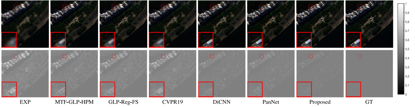
Fig. 4. Fusion results on the reduced resolution (simulated) Rio dataset (source: WorldView-3). Top row: the visual performance of the EXP, MTF-GLP-HPM, GLP-Reg-FS, CVPR19, DiCNN, PanNet, Proposed method, and the GT image, respectively. Bottom row: the corresponding MAE maps using the GT image as reference. For a better visualization, we doubled the intensities of the MAE maps and added 0.5.
