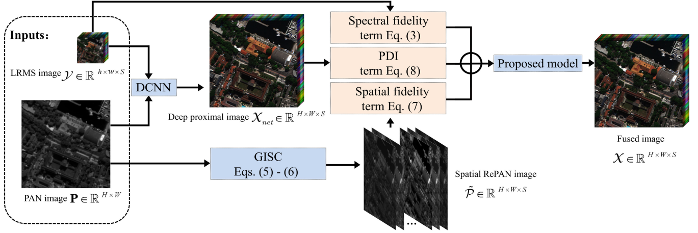
Fig. 2. Flowchart of our model. The GISC denotes the operation as in (5) and (6), see Section III-B. The acronym DCNN stands for deep convolutional neural network.
