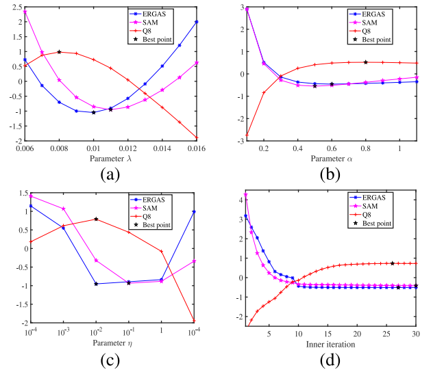
Fig. 9. ERGAS, SAM, Q8 curves for: the regularization parameters (a) \lambda and (b) \alpha , (c) the penalty parameter \eta and (d) the inner iteration p_{mit} . The best points are pointed out with a black star. Note that for better comparisons, we process the obtained indexes by (index - \mathcal{M}(index))/\mathcal{S}(index) , where \mathcal{M}(\cdot) and \mathcal{S}(\cdot) represent the mean and standard deviation operations, respectively. Besides, the real mean and standard deviation for ERGAS, SAM and Q8 are (a) 3.6479 \pm 0.0156 ; 4.0454 \pm 0.0131 ; 0.8714 \pm 0.0021 ; (b) 3.7763 \pm 0.3106 ; 4.1580 \pm 0.2309 ; 0.8667 \pm 0.0124 ; (c) 3.6747 \pm 0.0392 ; 4.1331 \pm 0.1090 ; 0.8706 \pm 0.0027 ; (d) 3.6400 \pm 0.0008 ; 4.0346 \pm 0.0094 ; 0.8720 \pm 0.0004 ; respectively.
