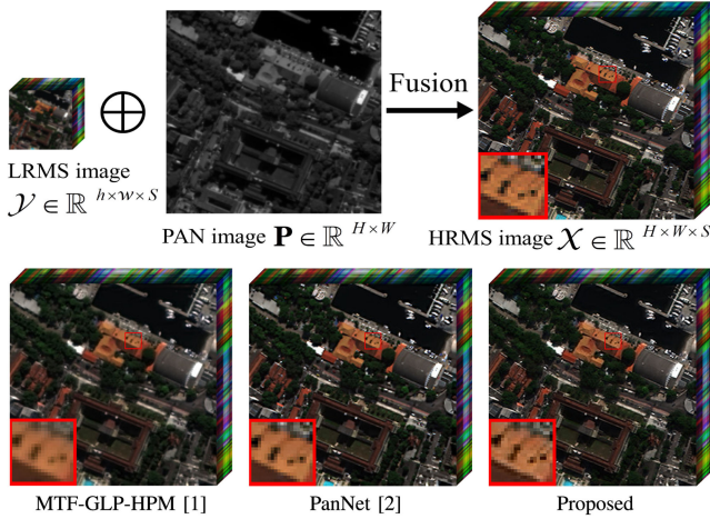
Fig. 1. Top row: the schematic of the PAN/MS fusion on a simulated Rio data (source: WorldView-3). Bottom row: fused images by the MTF-GLP-HPM [1], the PanNet [2] and the proposed method, respectively. The red, green, and blue channels of the shown images are extracted from the fifth, the third, and the second bands, respectively. Note that, the HRMS image \mathcal{X} displayed in the top row is the GT image.
