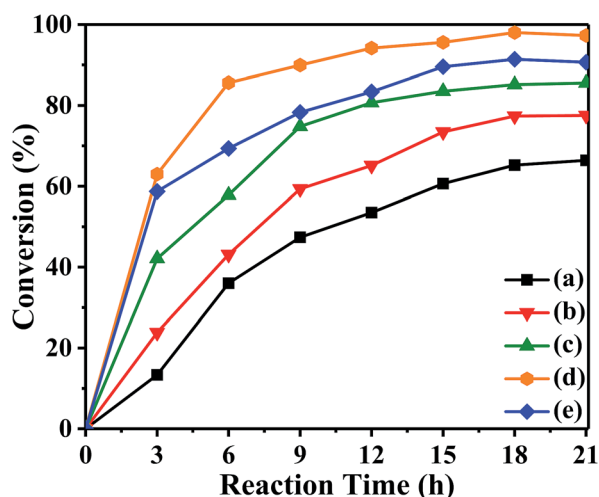
Fig. 7 The catalytic activities of prepared catalysts (a) blank, (b) the pristine UiO-67-bpy, (c) UiO-67- \text{H}_2\text{SO}_4 , (d) UiO-67- \text{CF}_3\text{SO}_3 , (e) UiO-67-hfp \text{OSO}_3 . Reaction conditions: catalyst amount 0.2 g, isooctyl alcohol to acetic acid molar ratio 1 : 6, at 80 °C.
