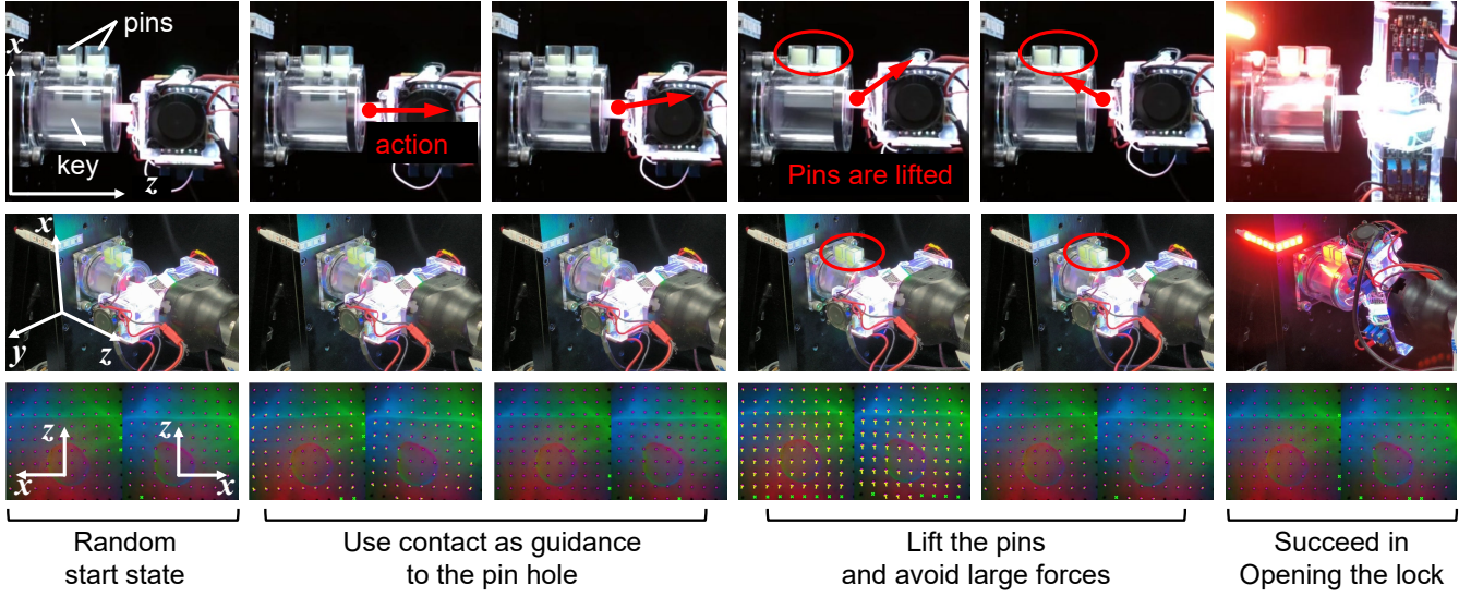
Fig. 19. The execution of lock opening task in reality. Real experimental setup and the definition of axial directions are shown in the first column. Tactile images from the sensors are shown in the bottom row. The actions are plotted in the top row as red arrows. The procedure can be divided into 4 stages: Start stage, Search stage, Lift stage and Finish stage. In Start stage, the start position is randomized. In Search stage, the key maintains contact with the lock core until the contact disappears. In Lift stage, the key is lifted and large contact forces should be avoided. Finally, in Finish stage, a manually-designed rotating motion is executed to turn the lock.
