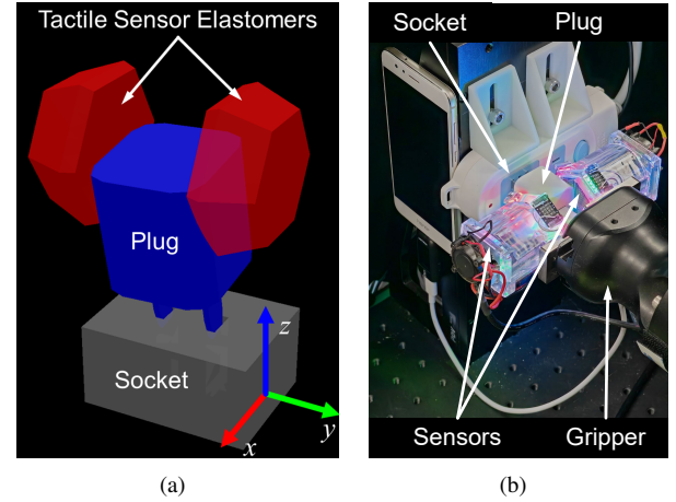
Fig. 17. The simulation setup and real setup of the plug adjustment task.
