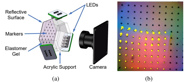
Fig. 2. (a) The schematic of the marker-based visuotactile sensor used in our work, which is based on GelSight [25]; (b) One example of real tactile image with marker tracking. The marker flow in contact area is shown by yellow arrows.
