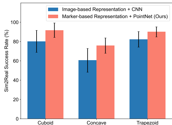
Fig. 14. Ablation study of the proposed tactile representation. Comparison is done between the proposed marker-based tactile representation and the image-based presentation. The success rates are compared over 3 test shapes. The average success rate and standard deviation are calculated from 10 independently trained weights for each representation.
