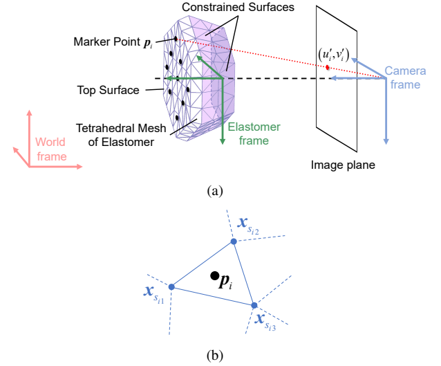
Fig. 3. (a) In our tactile sensor, the markers are distributed on the top surface. The surfaces in purple are constrained by the shell. The elastomer frame is fixed on the constrained surfaces of the elastomer. After transforming the marker point into the camera frame, one can calculate its pixel coordinate using the pinhole model. (b) Illustration of interpolation using adjacent FEM vertices. p_i denotes the i th marker, and the facet it belongs to has 3 vertices: x_{s1} , x_{s2} and x_{s3} .
