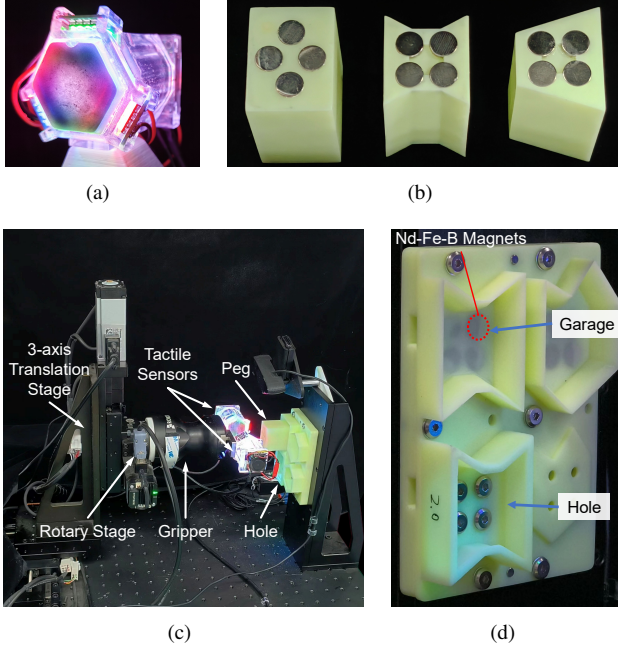
Fig. 10. The devices for the peg-in-hole experiment. (a) Our self-made GelSight-type tactile sensor. (b) These 3 shapes, namely Cuboid , Concave and Trapezoid , are used to test the trained policy in reality. The magnets are used for pose resetting. (c) We use a combined motorized stage and a parallel gripper to execute the tasks. (d) The mechanism for auto-resetting the pose. The garage has large chamfers to tolerate possible peg pose errors. There are also magnets at the bottom of the garage for pose resetting.
