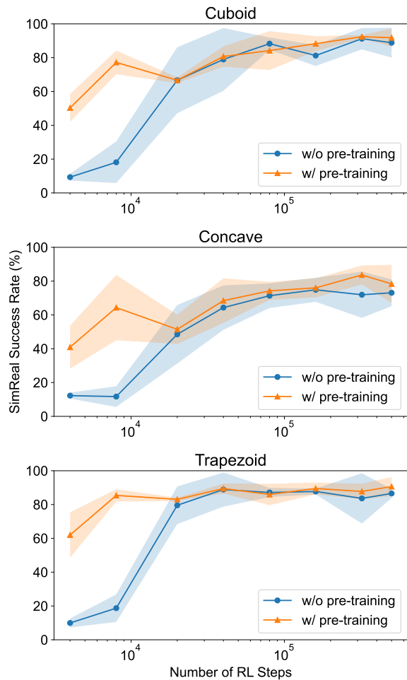
Fig. 15. Comparison between the policy with pre-training and without pre-training. Sim2Real success rates at different RL steps on 3 preset peg shapes are reported and each line is averaged over 3 weights trained with different random seeds. The horizontal axes are in log scale.
