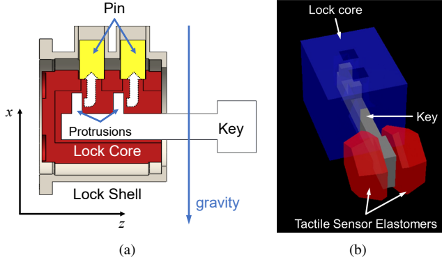
Fig. 18. The lock opening task. (a) The structure of the lock. With the protrusions on the key, it can lift the pins up and thus unlock the lock core. (b) In the simulation scene, the lock core is simplified.
