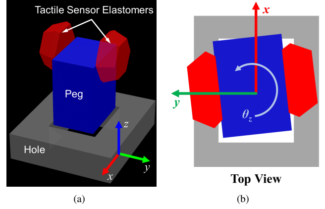
Fig. 9. (a) Our simulation environment of the peg-in-hole insertion task. Visualization is realized by SAPIEN [46]. (b) Top view of the task. The initial pose error has 3 degrees of freedom.
