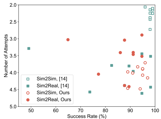
Fig. 16. Comparison of the Sim2Sim and Sim2Real results of our method and [14]'s method on the original peg-in-hole insertion task. The metrics are the success rate (higher is better) and the number of attempts (lower is better).
