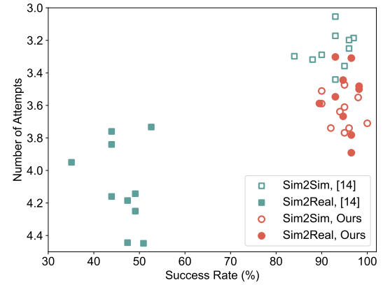
Fig. 11. Distribution of all the Sim2Sim and Sim2Real results of our method and [14]’s method on the monotone peg-in-hole insertion task. The metrics are the success rate (higher is better) and the number of attempts (lower is better). Our method has a higher success rate and a smaller Sim2Real gap.
