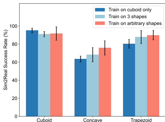
Fig. 13. Ablation study of the proposed arbitrary-shape training scheme. Comparison is done among training with arbitrary shapes, training with the exact 3 shapes and training with only one shape. The policy trained with arbitrary shapes has the best overall performance. This proves that a ‘generalist’ policy performs better in unknown environments and in Sim2Real.
