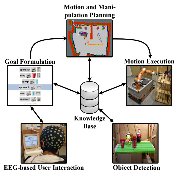
Figure 1: Our framework that unifies decoding of neuronal signals, high-level task planning based on referring expressions, low-level motion- and manipulation-planning, and scene perception with a centralized knowledge base at its core. Intuitive goal selection is provided through an adaptive graphical user interface.
