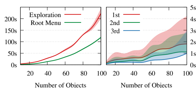
Figure 10: Evaluation of the computation time for different numbers of objects in the environment averaged over random actions. Left: The plot shows the mean and standard deviation of building the menu structure at the beginning and includes initial exploration and root menu creation. Right: Refinements of a goal can be done efficiently. It shows the mean and positive standard deviation times of the first three refinements.
